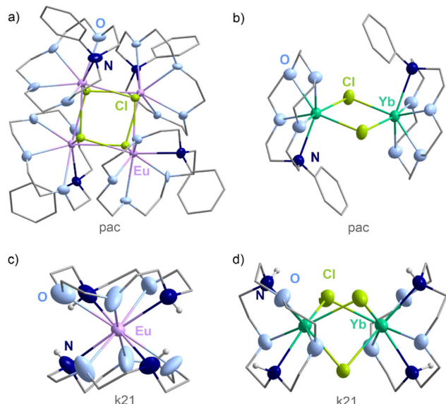
Fig. 4 Structure of (a) [\text{Eu}_4\text{Cl}_4(\text{pac})_4]^{4+} cation in 4 , (b) [\{\text{Yb}(\text{pac})\}_2(\mu\text{-Cl})_2]^{2+} cation in 5 , (c) [\text{Eu}(\text{k}21)_2]^{2+} cation in 10 , (d) [\{\text{Yb}(\text{k}21)\}_2(\mu\text{-Cl})_3]^+ cation in 11 (unit cells displayed in SI: Fig. S6, S7, S12 and S13).
