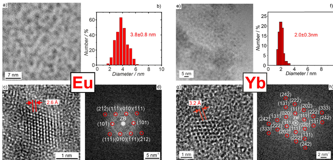
Fig. 2 Size and size distribution of the Eu(0) and Yb(0) nanoparticles: (a) and (e) TEM overview image, (b) and (f) size distribution based on a statistical evaluation of > 200 nanoparticles on TEM images, (c) and (g) HRTEM image of a single Eu(0)/Yb(0) nanoparticle with lattice fringes, (d) and (h) FT pattern of the single nanoparticle shown in (c) and (g). Red circles indicate the diffraction pattern of hexagonal bulk europium in the [101] zone axis (d) and of cubic bulk ytterbium in the [101] zone axis (h) (zero-order beam (ZB) marked by a white circle).
