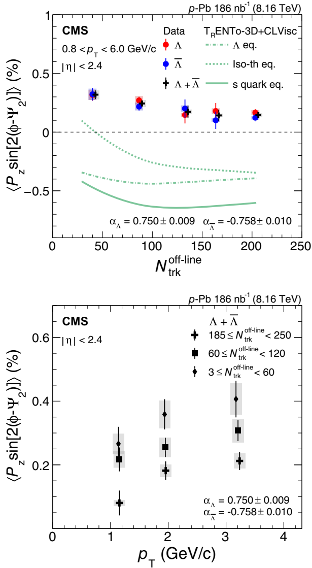
FIG. 2. Upper panel: The second-order Fourier sine coefficients of \Lambda , \bar{\Lambda} and \Lambda + \bar{\Lambda} polarizations along the beam direction as functions of N_{\text{trk}}^{\text{off-line}} in p\text{-Pb} collisions at \sqrt{s_{\text{NN}}} = 8.16 \text{ TeV} . Results from hydrodynamic calculations [66] are shown as solid and dashed lines. The N_{\text{trk}}^{\text{off-line}} values of \Lambda + \bar{\Lambda} results are shifted horizontally for better visibility. Lower panel: The second-order Fourier sine coefficients \Lambda + \bar{\Lambda} polarization along the beam direction as functions of p_T for 3 \leq N_{\text{trk}}^{\text{off-line}} < 60 , 60 \leq N_{\text{trk}}^{\text{off-line}} < 120 , and 185 \leq N_{\text{trk}}^{\text{off-line}} < 250 in p\text{-Pb} collisions at \sqrt{s_{\text{NN}}} = 8.16 \text{ TeV} . Vertical bars represent statistical uncertainties, while shaded areas show systematic uncertainties.
