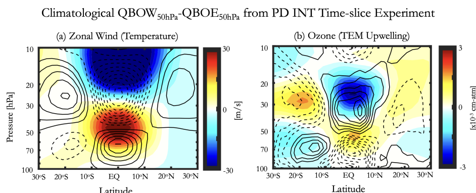
Figure 4. QBO westerly minus QBO easterly composites in zonal wind (colors) and temperature (black contours, 0.5 K interval) (a) derived from the GISS E2-2 PD-INT time-slice experiment. (b) Same as in (a), except for ozone (colors) and residual mean upwelling (black contours, 2 \times (10^{-7}) mb/s). The QBO has been evaluated at 50 hPa.
