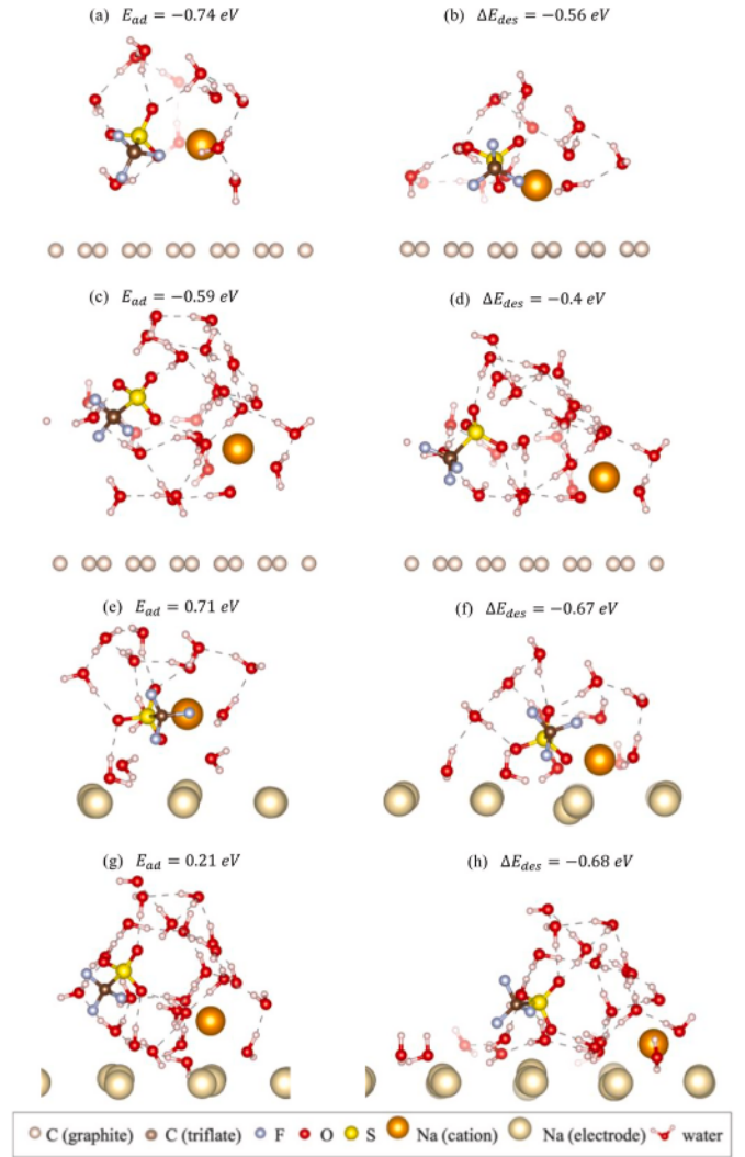
Fig. 6. Structures of contact and solvent-separated ion pair models in proximity to the examined surfaces: a-d) 3 layers of graphite, and e-h) a 4-layer bcc (100) sodium surface. The panels show fully solvated contact (a and e) and solvent-separated (c and g) ion pair structures, as well as partly desolvated contact (b and f) and solvent-separated (d and h) ion pair structures. For the fully solvated adsorbates, the corresponding panels display the adsorption energies, E_{ad} , obtained from Eq. (1), and for the partly desolvated adsorbates, the panels show the desolvation energies, \Delta E_{des} , approximated from Eq. (3).
