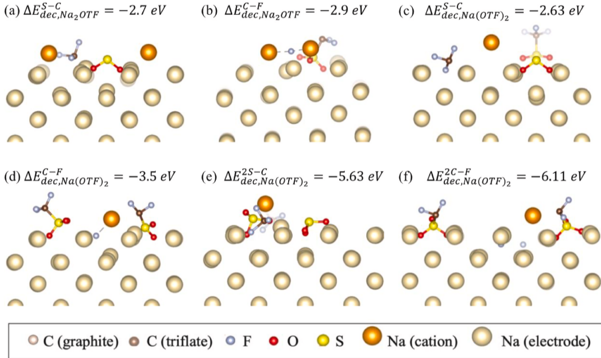
Fig. 5. Structures of potential decomposition products of triflate anion(s) during adsorption of \text{Na}_2\text{OTF} and \text{Na}(\text{OTF})_2 aggregates on a bcc (100) sodium surface. These structures represent the breaking of: a) the S-C bond in \text{Na}_2\text{OTF} , b) one C-F bond in \text{Na}_2\text{OTF} , c) one S-C bond in \text{Na}(\text{OTF})_2 , d) one C-F bond in \text{Na}(\text{OTF})_2 , e) both S-C bonds in \text{Na}(\text{OTF})_2 , and f) two C-F bonds from different anions in \text{Na}(\text{OTF})_2 . Each panel displays the corresponding decomposition reaction energy, \Delta E_{dec} , obtained from Eq. (2).
