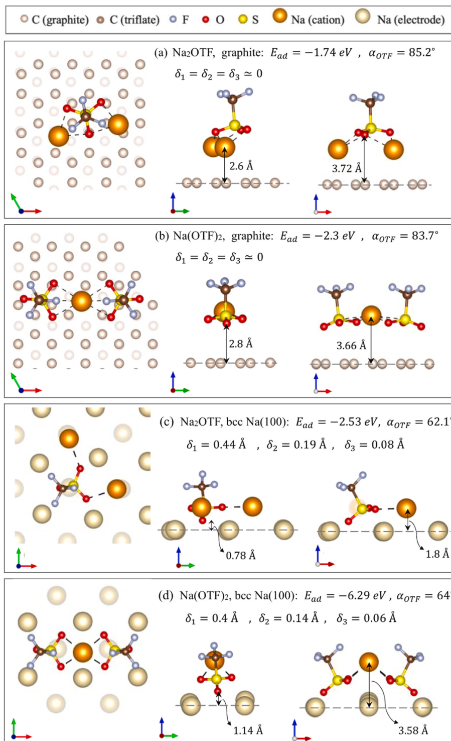
Fig. 4. Top and side views of the adsorption structures of multi-ion complex models on the examined surfaces: a) \text{Na}_2\text{OTF} on 3 layers of graphite, b) \text{Na}(\text{OTF})_2 on 3 layers of graphite, c) \text{Na}_2\text{OTF} on a 4-layer bcc (100) sodium surface, and d) \text{Na}(\text{OTF})_2 on a 4-layer bcc (100) sodium surface. Each panel displays the corresponding adsorption energy, E_{ad} , obtained from Eq. (1), alongside key structural properties: the vertical distance between the sodium cation and the average position of atoms in the topmost surface layer, the vertical distance between the nearest oxygen atom of the triflate anion(s) to the surface and the average position of atoms in the topmost surface layer, r_{\text{O-C}} or r_{\text{O-Na}} , the angle between the S-C bond in the triflate anion and the surface plane, \alpha_{\text{OTF}} , and the maximum atomic displacements in surface layers relative to the bare surface ( \delta_1 for the topmost layer, \delta_2 for the second layer, and \delta_3 for the third layer).
