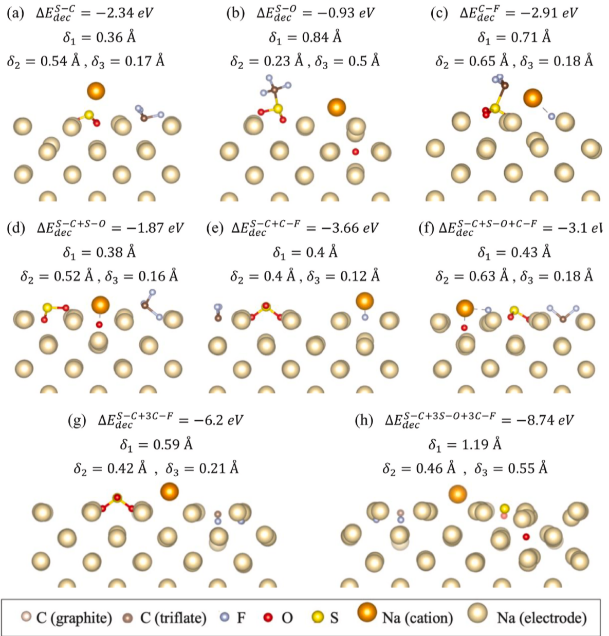
Fig. 3. Potential adsorption structures of a NaOTf ion pair on a 4-layer bcc (100) sodium metal surface considering different anion decomposition scenarios. The decomposition products correspond to the breaking of: a) the S-C bond, b) one S-O bond, c) one C-F bond, d) the S-C plus one S-O bond, e) the S-C plus one C-F bond, f) the S-C plus one S-O plus one C-F bond, g) the S-C plus three C-F bonds, and h) the S-C plus three S-O plus three C-F bonds. Each panel displays the corresponding decomposition reaction energy ( \Delta E_{dec} ) obtained from Eq. (2), and the maximum atomic displacements in surface layers relative to the bare surface ( \delta_1 for the topmost layer, \delta_2 for the second layer, and \delta_3 for the third layer).
