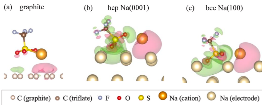
Fig. 2. Charge rearrangements induced by the adsorption of a NaOTF ion pair on the examined surfaces: a) 3 layers of graphite, b) a 4-layer hcp (0001) sodium surface, and c) a 4-layer bcc (100) sodium surface. The figure displays the electron density difference using two isosurfaces (red: +0.001 e/ \text{\AA}^3 and green: -0.001 e/ \text{\AA}^3 ), showing the difference between the electron density of the adsorption complex and that of the isolated ion pair and the bare surface. (For interpretation of the references to colour in this figure legend, the reader is referred to the Web version of this article.)
