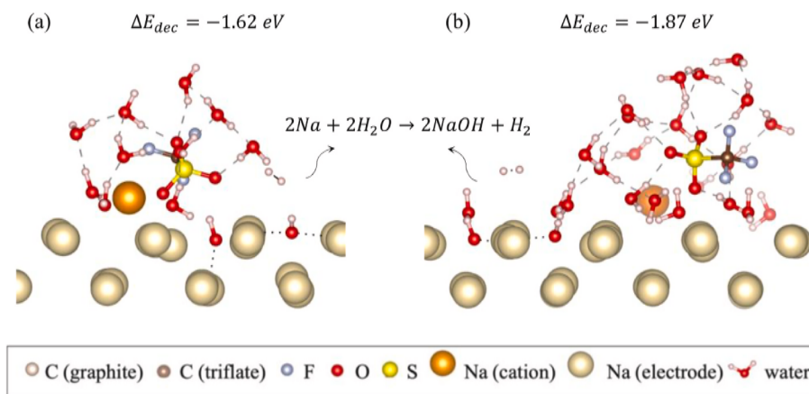
Fig. 7. Exemplary water decomposition products resulting from the reduction of water molecules approached a 4-layer bcc (100) sodium surface as part of adsorbed contact (panel a) and solvent-separated (panel b) ion pair structures. Each panel displays the corresponding decomposition reaction energy, \Delta E_{dec} , obtained from Eq. (2) with respect to the adsorption complexes containing intact water molecules.
