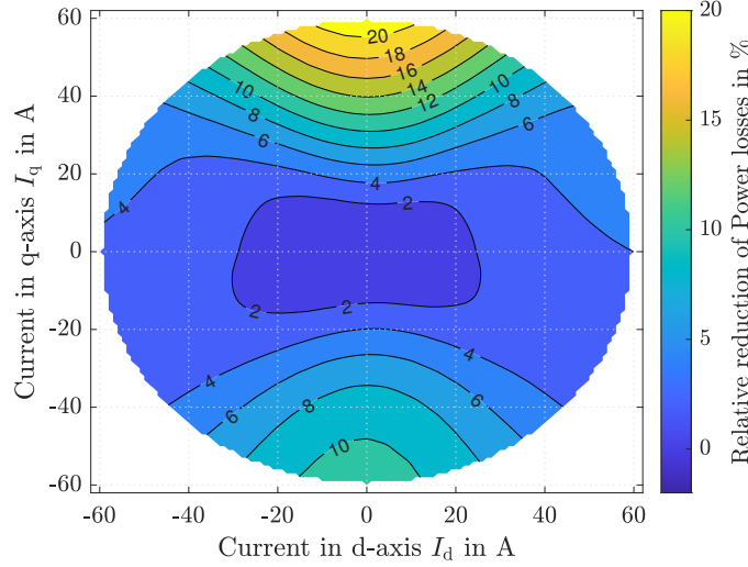
Fig. 19: Calculated relative reduction of the losses of the DAB stages.
