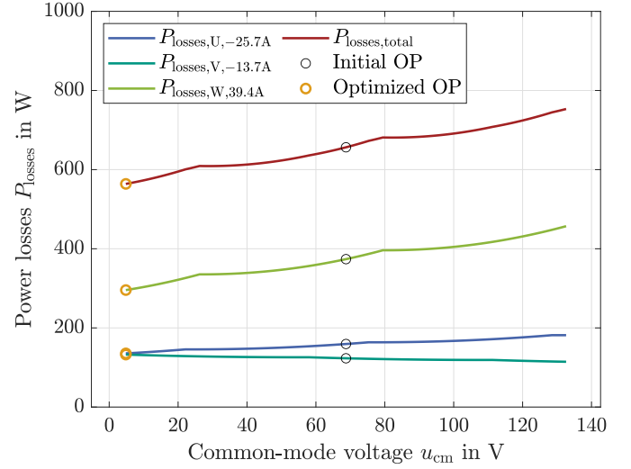
Fig. 7: Losses within each phase and total DAB losses in relation to the valid CM voltage u_{cm} range. ( \hat{u}_{AC} = 325 V, \hat{i}_{AC} = 40 A, \varphi = 65^\circ , \gamma = 25^\circ )
