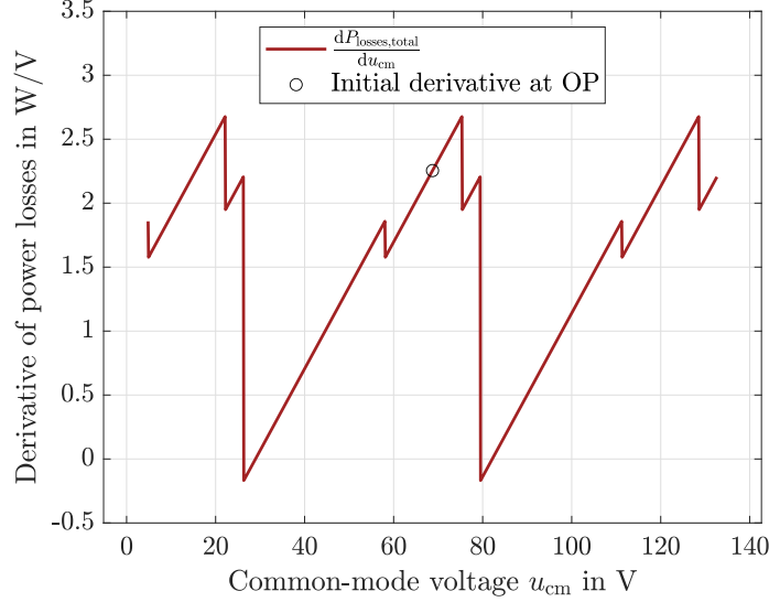
Fig. 9: Derivative of total power losses \frac{dP_{\text{losses},\text{total}}}{du_{\text{cm}}} with respect to the residual CM voltage u_{\text{cm}} range ( \hat{u}_{\text{AC}} = 325 \text{ V} , \hat{i}_{\text{AC}} = 40 \text{ A} , \varphi = 65^\circ , \gamma = 25^\circ ).
