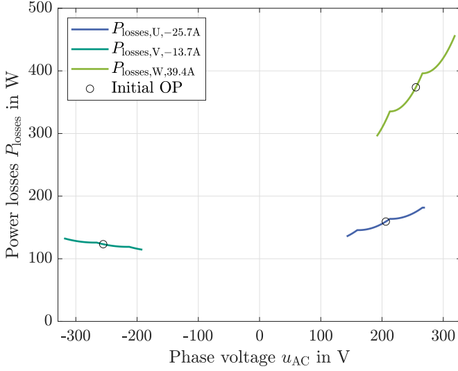
Fig. 6: Calculated power losses of each phase for a specific OP and valid voltage modification range. ( \hat{u}_{AC} = 325 V, \hat{i}_{AC} = 40 A, \varphi = 65^\circ , \gamma = 25^\circ )
