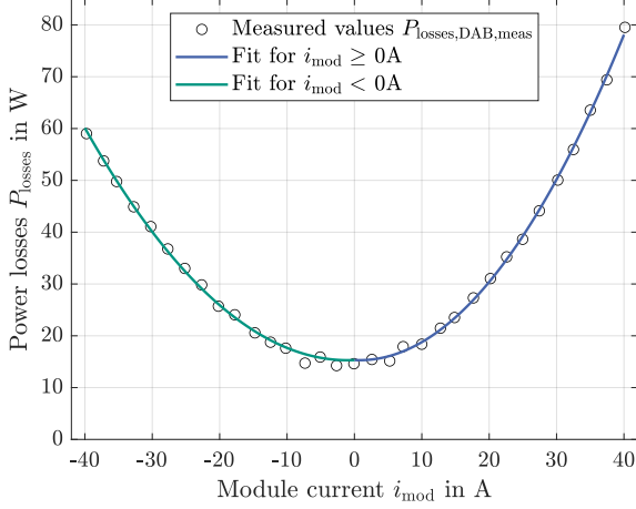
Fig. 4: Measured and fitted power losses of a DAB with U_p = 750 V and U_{mod}^* = 53.2 V.
