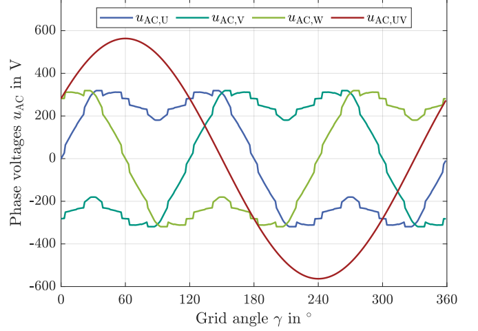
Fig. 15: Resulting calculated, switching period average SST output phase voltages with loss optimized CM voltage. Resulting sinusoidal line-to-line voltage u_{\text{AC},\text{UV}} between phases U and V.
