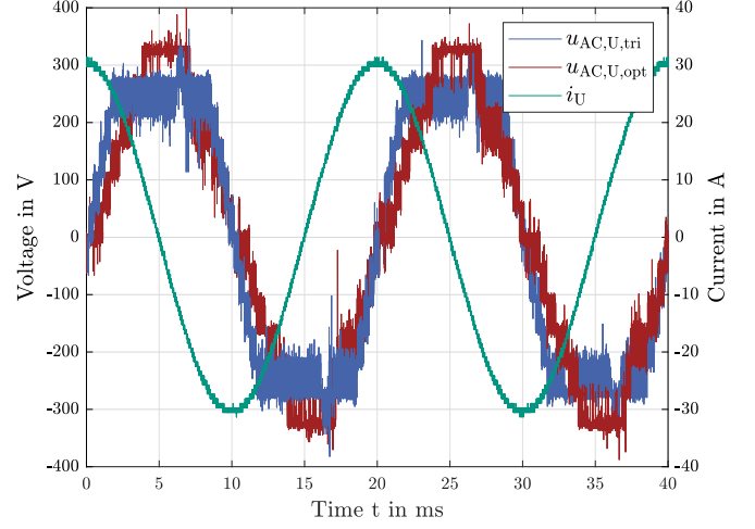
Fig. 17: Measured reference (blue) and optimized (red) voltage and current (green) of phase U with I_d = 0 A and I_q = 30 A.
