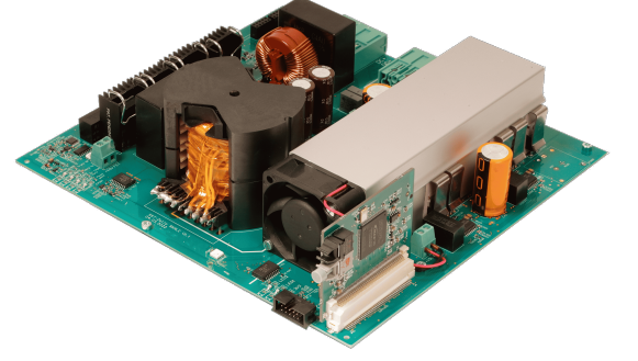
Fig. 10: Hardware of the power module with a DAB stage and the CHB cell.
