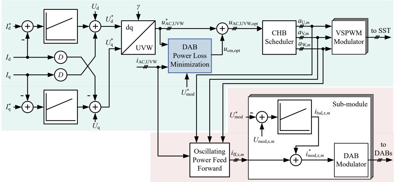
Fig. 11: Employed control structure for the SST with AC-side current control (green) and DC-link voltage control (red). The proposed Power Loss Minimization Algorithm (blue) is integrated into the AC-side current control. Connections consisting of more than one signal are indicated by the three dashes.
