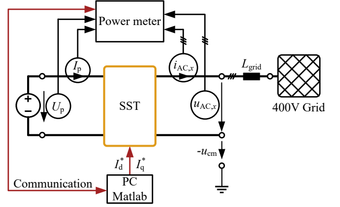
Fig. 13: Test setup to measure the losses of the SST during operation. Connections consisting of more than one signal are indicated by the three dashes.
