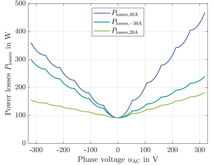
Fig. 5: Calculated power losses of a single phase with six modules for different phase currents and voltages.
