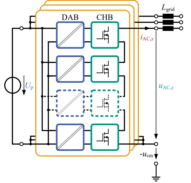
Fig. 3: Three-phase modular ISOP SST for AC/DC grid coupling. The dotted module indicates that multiple modules can be used.
