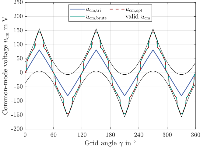
Fig. 14: Comparison of the valid CM voltage u_{\text{cm}} for a grid period.
