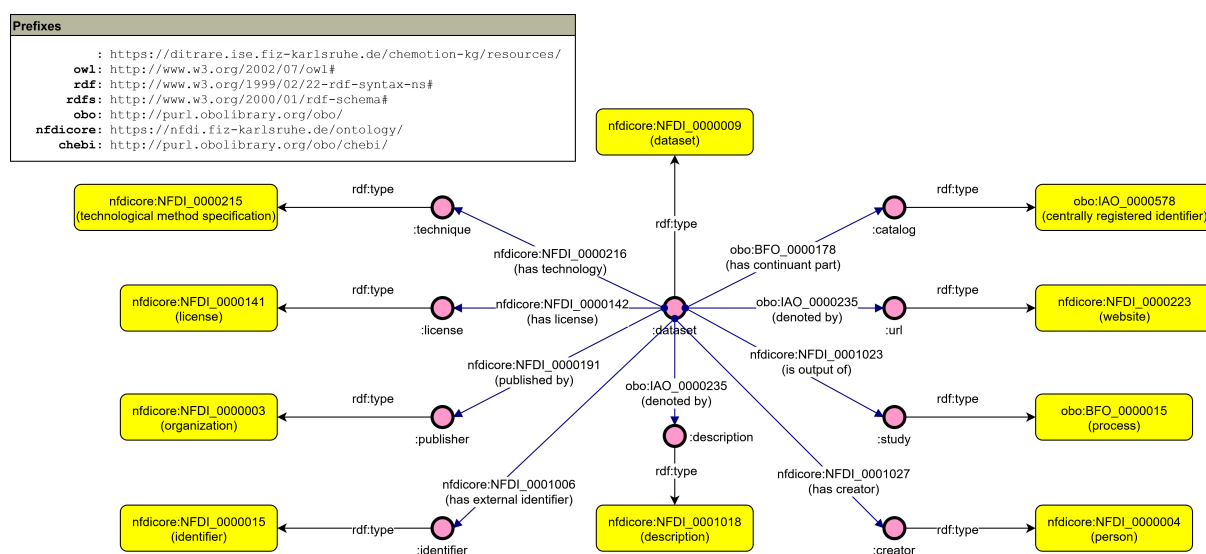
Figure 2: Dataset representation in the Chemotion-KG.
