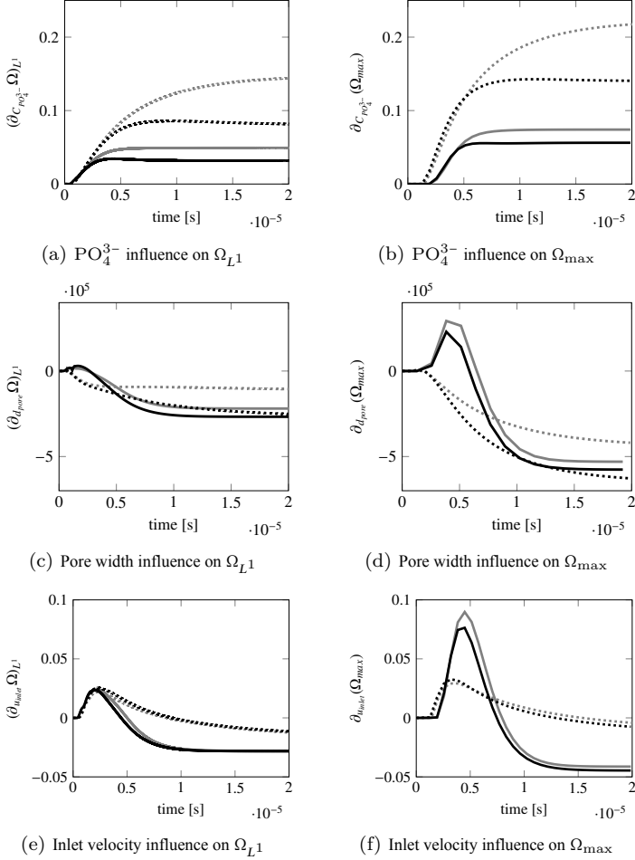
Figure 5.10.: Maximal and spatially averaged developments of saturation product \Omega and its derivatives with respect to surface potential \psi_{\text{H}} , hydrogen and phosphate concentrations \text{H}^+ , \text{PO}_4^{3-} , pore width and inlet carrier fluid velocity u_{\text{in}} on the a) and b) geometries by opposite Helmholtz potentials of \pm 0.01 V. Part II/II.
