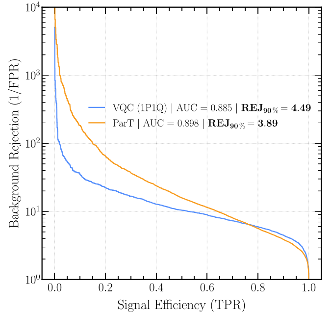
FIG. 5. Comparison of ROC curves for the VQC and particle transformer. The VQC trained on the 1P1Q-encoded dataset closely matches the performance of the state-of-the-art particle transformer, despite using significantly fewer trainable parameters, with both being trained on the same number of events and input size of 10 particles.
