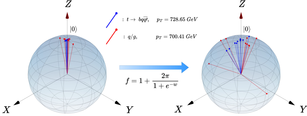
FIG. 1. Bloch sphere: Effect of the input scaling described in Eq. (4) when applied to the ten hardest particles of a QCD and top jet with comparable jet p_T . The value of w converges to a scaling factor f = 7.268 for the VQC.
