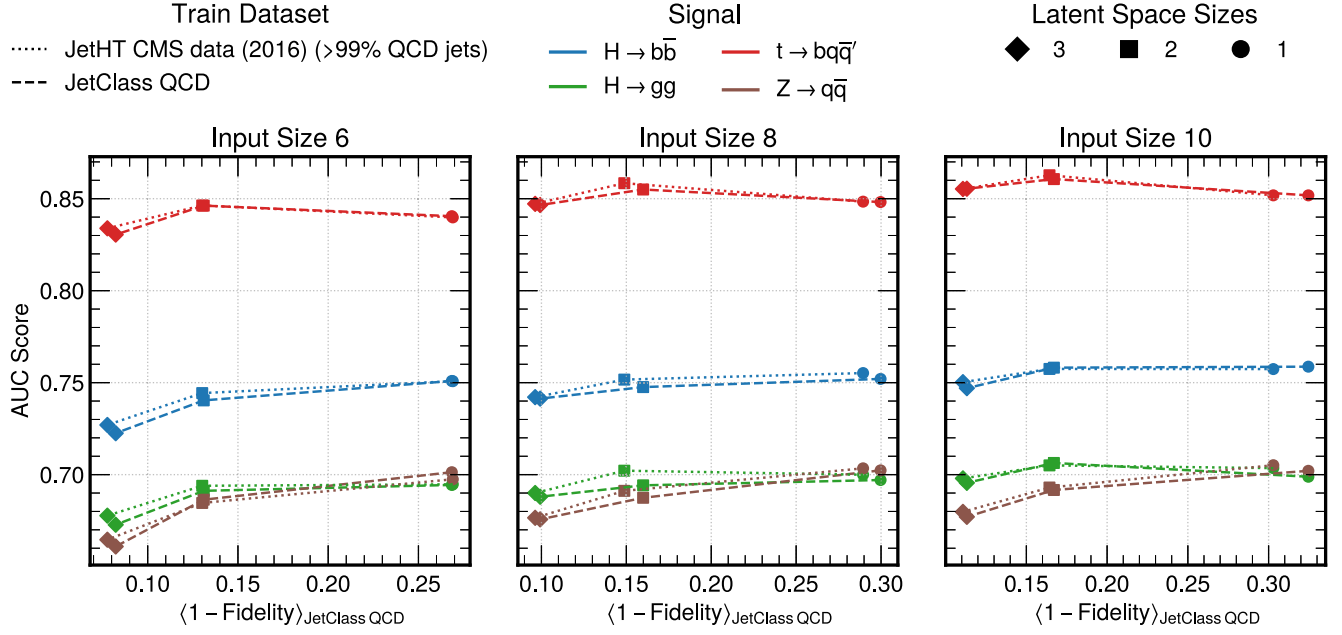
FIG. 4. AUC scores vs \langle 1 - \text{Fidelity} \rangle_{\text{QCD}} for different QAE configurations. Models trained on simulated (dashed) and real CMS data (dotted) show consistent trends, with larger input sizes and higher fidelity loss correlating with improved anomaly detection performance.
