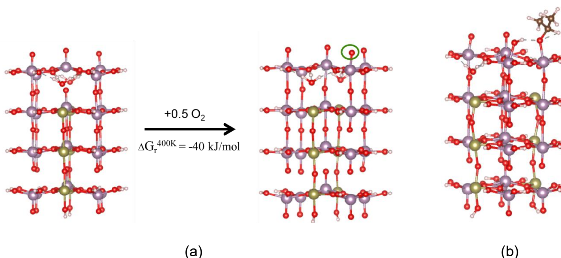
Figure 6.9. (a) Te free Mo-only active site can thermodynamically have three metal-oxo sites, as shown here. (b) The presence of neighboring metal-oxo sites facilitates isopropanol generation, via the two-step mechanism, such as first by adsorbing propyl radical strongly and then fast H-migration from neighboring M-OH site towards it as shown here.
