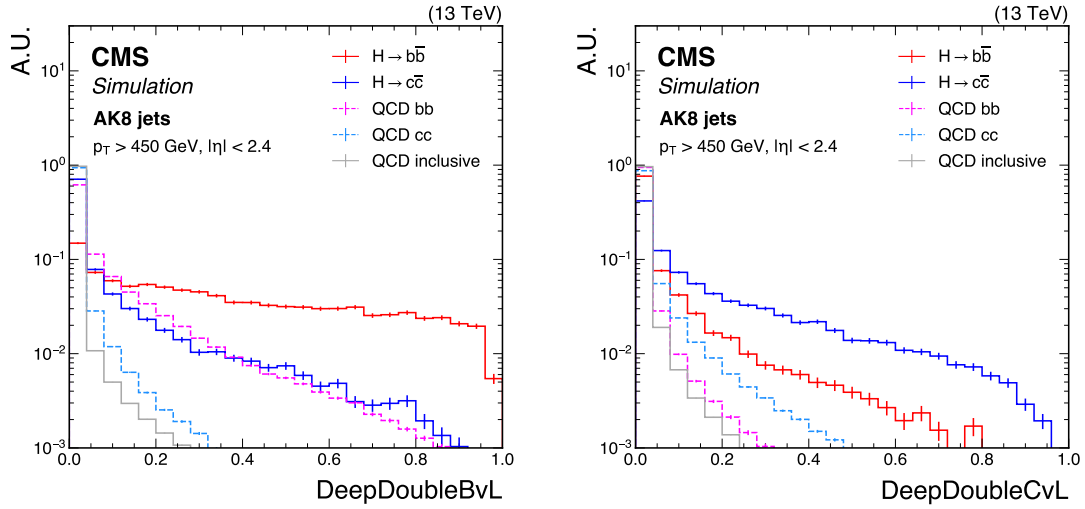
Figure 2. Shape comparison of the DeepDoubleBvL (left) and DeepDoubleCvL (right) discriminants for the simulated standard model H \rightarrow b\bar{b} and H \rightarrow c\bar{c} jets, the b\bar{b} and c\bar{c} components of QCD multijet background jets, and inclusive QCD jets, using simulated events corresponding to the 2018 data-taking conditions for jets with p_T > 450 GeV and |\eta| < 2.4 . The error bars represent the statistical uncertainties due to the limited number of simulated events.
