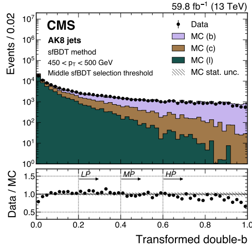
Figure 16. An example of the transformed double-b distribution in data and simulated events, after applying the preselection and the middle sfBDT selection threshold in the sfBDT method. The high-purity (HP), medium-purity (MP), and low-purity (LP) working points correspond to selections of X > 0.6, 0.4, 0.2 on the transformed tagger discriminant. The error bars represent the statistical uncertainties in observed data, which may be too small to be visible. The lower panel displays the ratio of data to simulation, with the hatched bands representing the normalized statistical uncertainty of simulated events for each bin. The distribution is based on data and simulated events with the 2018 data-taking conditions, in the jet p_T range of (450, 500) GeV.
