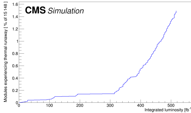
Figure 54. Fraction of modules affected by thermal runaway as a function of the integrated luminosity.
