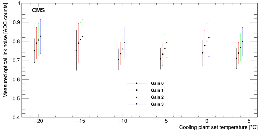
Figure 12. Noise measured in the optical link chain during optical link setup runs at temperatures between +4^\circ\text{C} and -20^\circ\text{C} coolant temperature for the four laser driver gain settings. The error bars show the root-mean-square (RMS) of the individual noise distributions and are a measure of the spread of the noise among all optical links in the SST. Points for different gain settings at the same temperature are slightly displaced for visibility.
