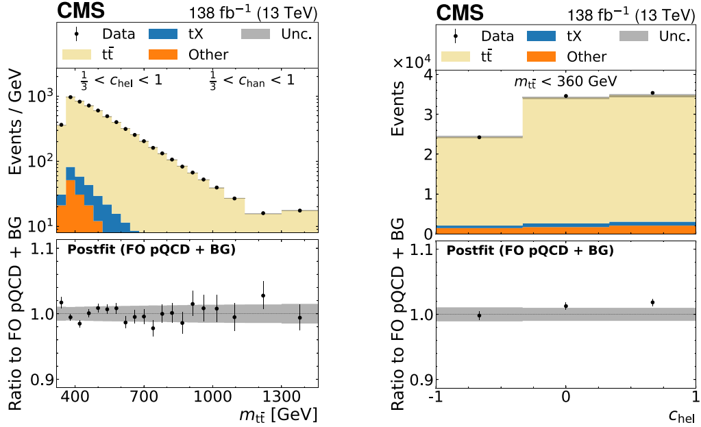
Figure 4. Observed (points with statistical error bars) and predicted (stacked colored histograms) m_{t\bar{t}} distribution in the (c_{\text{hel}}, c_{\text{chan}}) bin with the highest expected \eta_t contribution (left) and c_{\text{hel}} distribution for m_{t\bar{t}} < 360 GeV and integrated over c_{\text{chan}} (right). In the upper panels, the histograms account only for the FO pQCD + background prediction, and are shown after the background-only fit to the data. On the left, the shown event rates are divided by the bin width. The lower panels display the ratio of the data to the FO pQCD + background prediction. The gray band indicates the postfit uncertainty. The binning is the same as in figures 1 and 2 (left).
