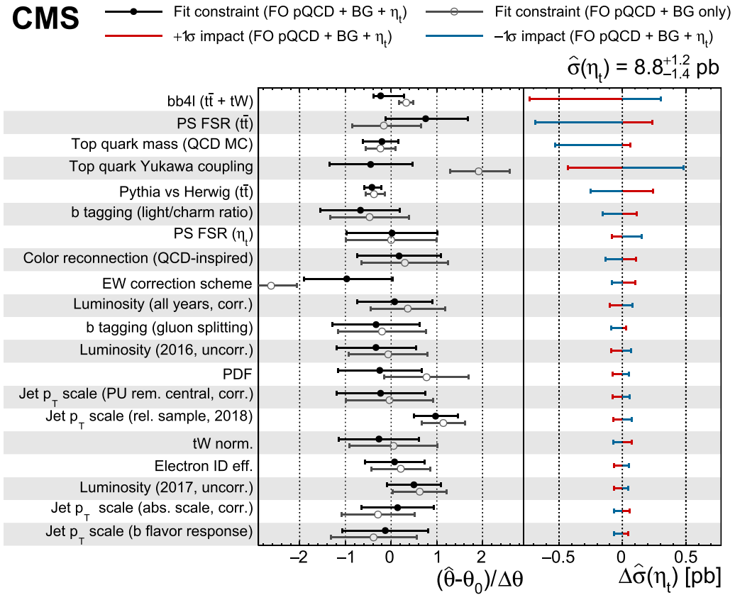
Figure 5. For the nuisance parameters listed in the left column, the pulls (\hat{\theta} - \theta_0)/\Delta\theta (middle column), where \hat{\theta} and \theta_0 are the postfit and prefit values of the nuisance parameters and \Delta\theta is the prefit uncertainty, are shown for the FO pQCD + background + \eta_t (black filled circles) and FO pQCD + background (gray empty circles) fit, as well as the impacts \Delta\hat{\sigma}(\eta_t) (right column) for the FO pQCD + background + \eta_t fit. The impact \Delta\hat{\sigma}(\eta_t) for a nuisance parameter \theta is calculated by varying \theta by \pm 1 SD and evaluating the shift in \sigma(\eta_t) . The nuisance parameters are ordered by the maximum of their \pm 1 SD impacts in the FO pQCD + background + \eta_t fit.
