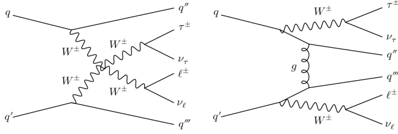
Figure 1. Representative tree-level Feynman diagrams contributing to the process qq' \rightarrow \tau^\pm \nu_\tau \ell^\pm \nu_\ell jj , \ell = e, \mu , leading to cross sections of order \alpha_{EW}^6 (left) and \alpha_S^2 \alpha_{EW}^4 (right).
