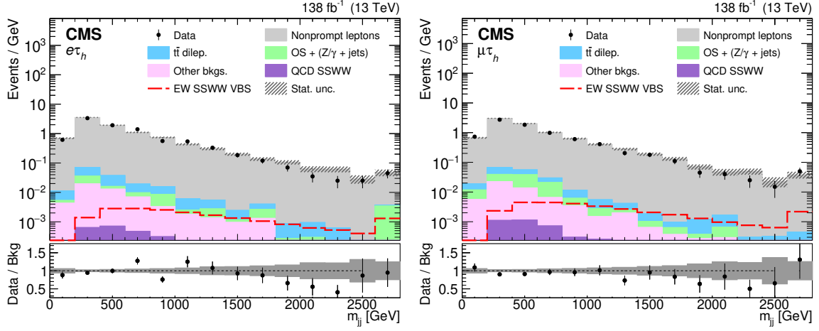
Figure 2. Distributions in the invariant mass of the dijet system for the data and the pre-fit background prediction for the (left) e\tau_h and (right) \mu\tau_h nonprompt VRs. The stacked filled histograms show the background components, with the overflow count included in the last bin. The expectation for the EW SSWW signal is shown by the dashed red line. The hatched error band shows the bin-by-bin statistical uncertainty. The lower panels show the ratio of data to the total background prediction, with statistical uncertainties indicated by error bars and shading, respectively. In all the panels, the vertical bars represent the statistical uncertainty assigned to the observed number of events.
