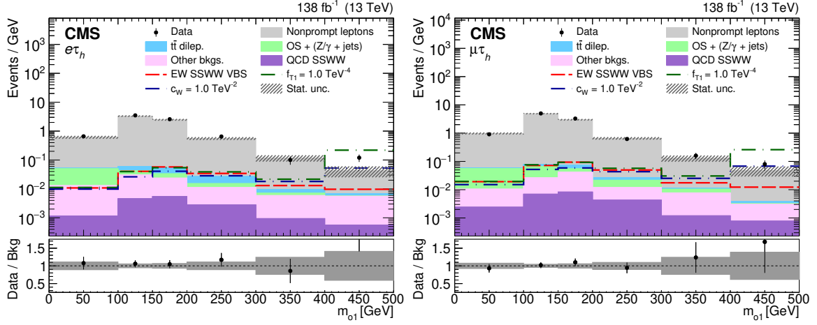
Figure 3. Distributions in m_{\tau_1} transverse mass for the data and the pre-fit background prediction for the (left) e\tau_h and (right) \mu\tau_h SRs. The stacked filled histograms show the background components, and the overflow count is included in the last bin. The expectations for the EW SSWW signal, the \mathcal{O}_W dim-6 operator with c_W = 1 \text{ TeV}^{-2} , and the \mathcal{Q}_{T1} dim-8 operator with f_{T1} = 1 \text{ TeV}^{-4} are shown by the dashed red, blue, and green lines, respectively. For the latter two, the interference with SM and pure EFT contributions are summed together with the SM contribution. The hatched error band shows the bin-by-bin statistical uncertainty. The lower panels show the ratio of data to the total background prediction, with statistical uncertainties indicated by error bars and shading, respectively. In all the panels, the vertical bars represent the statistical uncertainty assigned to the observed number of events.
