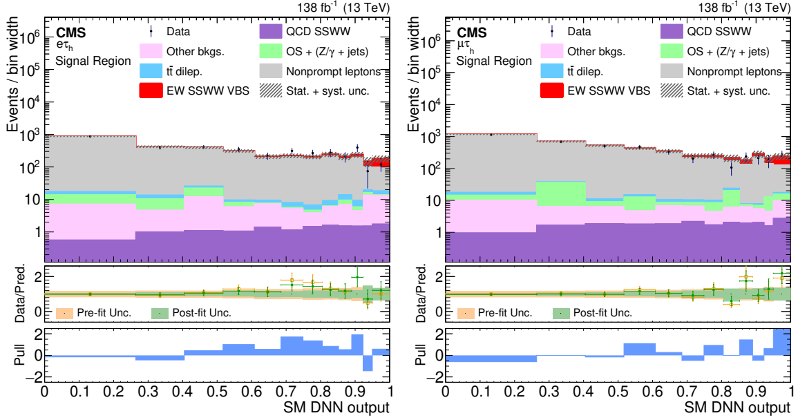
Figure 4. Distribution of the DNN output for the (left) e\tau_h and (right) \mu\tau_h SR. The data points are overlaid on the post-fit background plus signal (stacked histograms). The overflow is included in the last bin. The middle panels show ratios of the data to the pre-fit background prediction and post-fit background yield in yellow and green, respectively. The corresponding colored bands indicate the systematic component of the uncertainty. The lower panels show the distributions of the pulls, defined in the text. The vertical bars represent the statistical uncertainty assigned to the observed number of events for the upper panel, and its propagation to the quantities shown in the middle panel.
