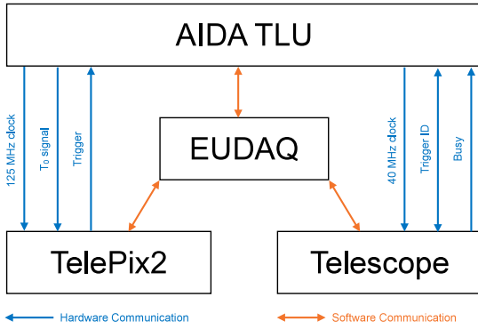
Fig. 4. Typical test beam setup. TELEPIX2 connects to a DUT interface of the AIDA-TLU and receives a 125 MHz clock and T_0 at run start while providing a trigger output. The MIMOSA telescope operates in the EUDET mode to exchange the trigger ID, while ADENIUM [14] runs in AIDA+trigger ID mode. EUDAQ2 is used to steer the data taking. External DUTs are not shown.
