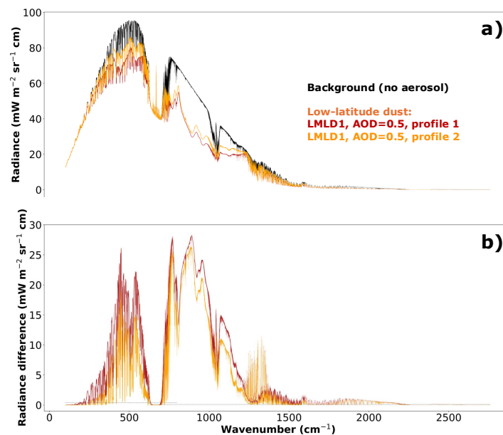
Figure 4: Merged FORUM and IASI-NG PO spectra for the case of Australia dust sample, with a FIR AOD=0.5, and the two different vertical profiles (profile 1, red curve: peaking at 5 km altitude; profile 2, yellow curve: peaking at surface) (a). A background spectrum, i.e. with the same configuration but without any dust layer, is shown as a black curve in panel a, as a baseline reference. Corresponding spectral signatures (b).
