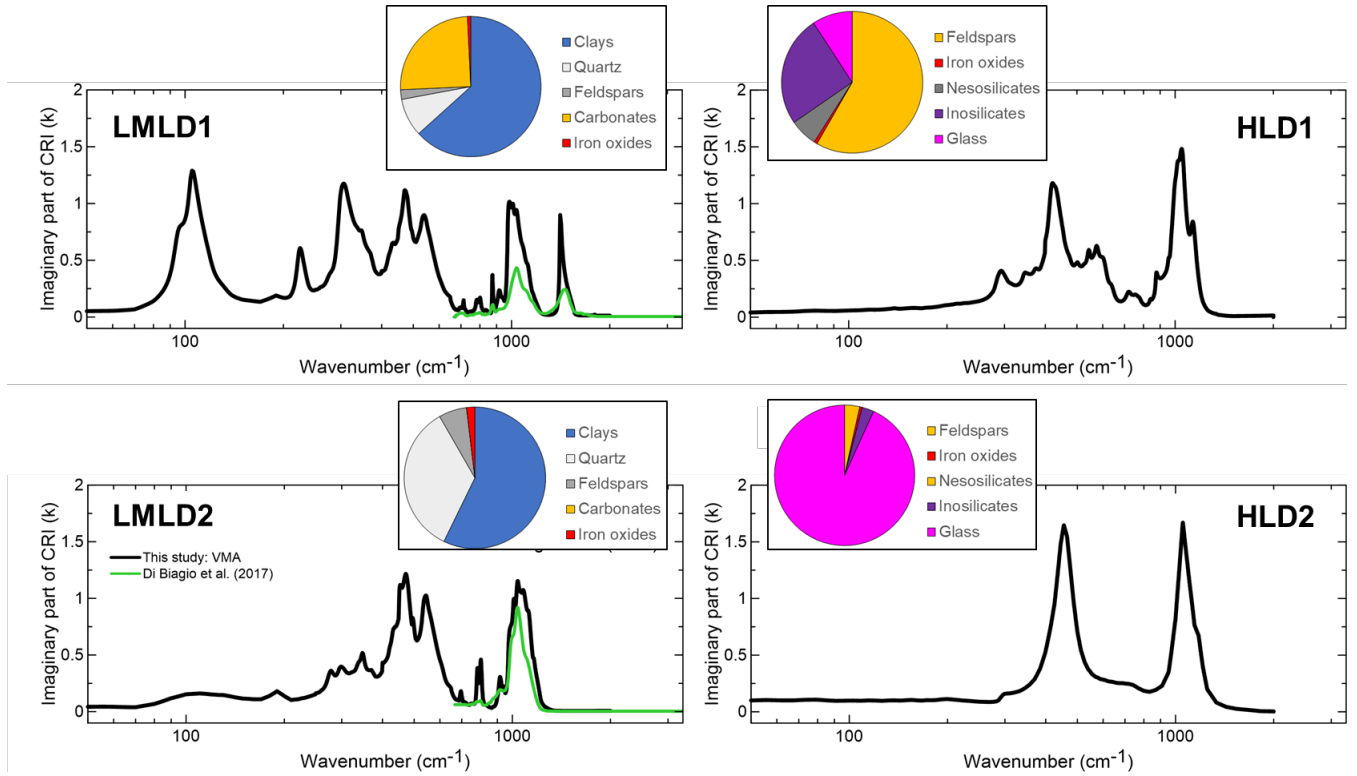
165 Figure 2: The spectral imaginary part of the complex refractive indices calculated using the VMA method (in black) compared with the experimental measurements from Di Biagio et al. (2017) for LMLD1 and LMLD2 (in green). The mineralogical composition (% in volume) of the four dust samples is also shown in the inlets. The spectral data for the real part of the CRI are shown in Supplementary Figure S2.
