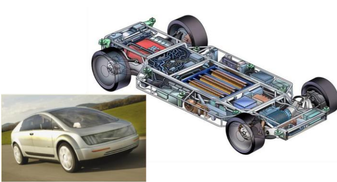
Abbildung 5-13: General Motors HY-Wire [Per-04]
