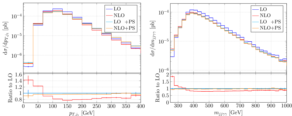
Figure 2. Distributions of the transverse momentum of the leading jet (left) and the invariant mass of the two b -jets and two photons (right), assuming the fiducial selection described in section 2.2. In each plot, the upper pane shows results with the production evaluated at LO; the H \rightarrow b\bar{b} decay is calculated either at LO or at NLO, and with or without PS. The lower pane of each plot shows the ratio of the different curves of the upper pane to the corresponding LO curve.
