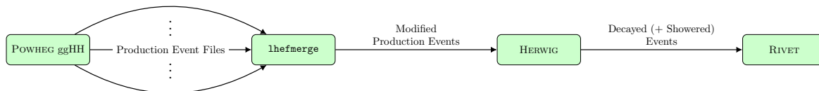
Figure 1. Workflow of the event generation and analysis setup.
