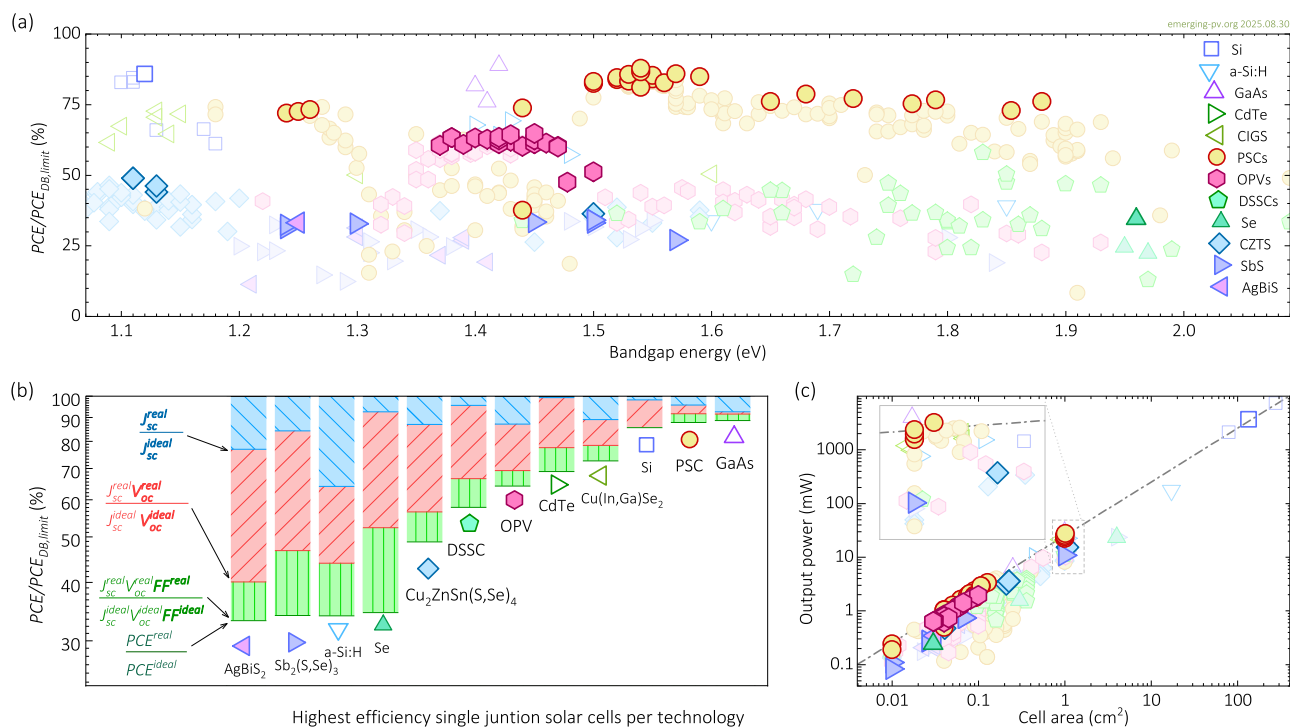
FIGURE 3 | Detailed balance efficiency limit analysis (a, b) and output power (c). (a) Experiment-to-detailed balance efficiency-limit ratio (EDBL, Equation 4, and in Table 2) as a function of the bandgap energy, based on the data in Figure 2. (b) Logarithmic loss analysis [16, 17] for the device with the highest PCE of each PV technology. (c) Output power versus device area, where the dash-dotted line represents the efficiency isoline for PCE = 25\% . In (a) and (c), opaque symbols correspond to reports published after August 2024, while light symbols denote earlier reports.
