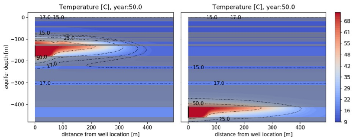
Figure 24. Numerical simulations depicting the temperature distribution after 50 years of HT-ATES operation for the Maassluijs Formation (left) and Ommelanden Formation (right) [17]. Reproduced with the permission of the International Geothermal Association and Dr. Martin Bloemendal.
