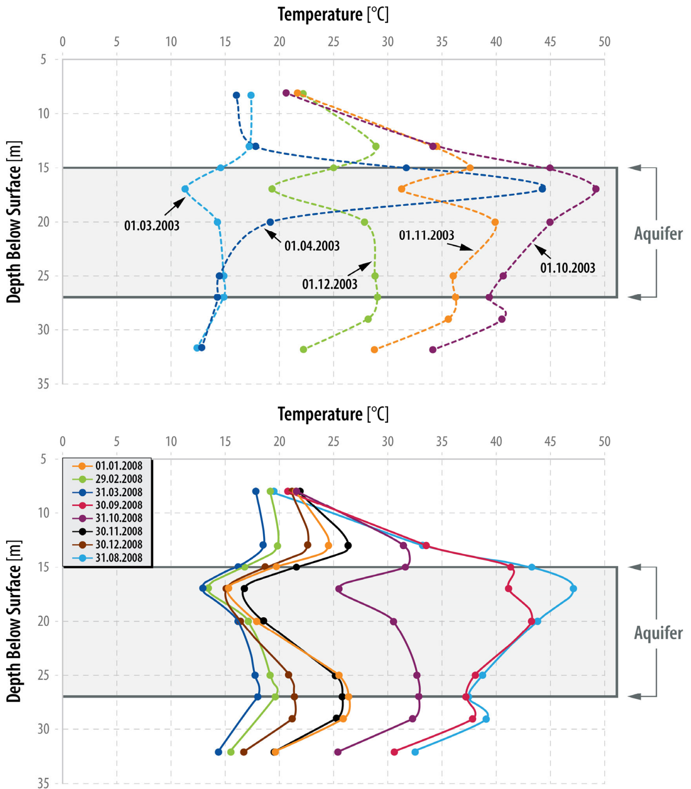
Figure 11. Measured temperatures in the Rostock HT-ATES aquifer at a distance of 5 m from the hot well in the groundwater flow direction at different dates in (a) 2003—[82] and (b) 2008—[85]. Reproduced with the permission of the Secretariat of the International Energy Agency Energy Storage TCP, the International Solar Energy Society, and Prof. Dr. Müller-Steinhagen.
