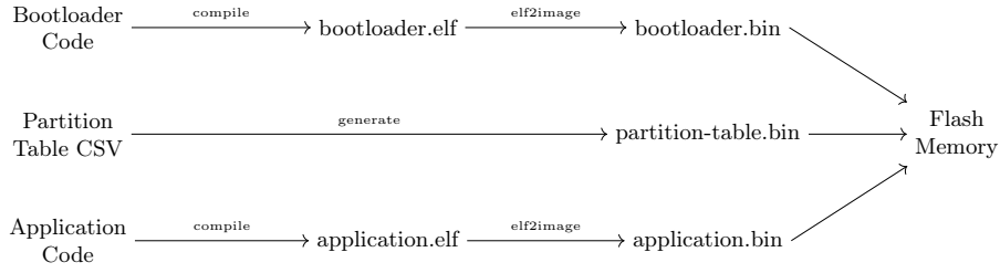
Fig. 1. The build and flash process
