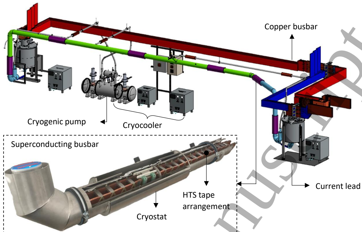
Figure 1: Superconducting busbar system for 20 kA next to a comparable copper busbar system
