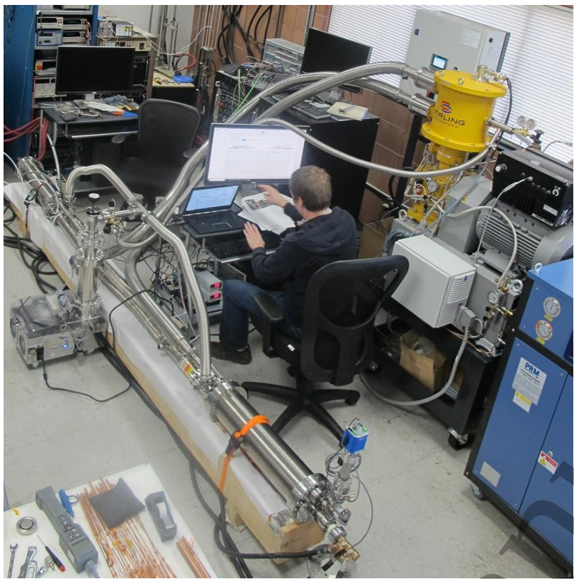
Figure 1: 20-30 K cooling loop set-up to cool DC cables Courtesy of Advanced Conductor Technologies LLC, Boulder CO, USA
