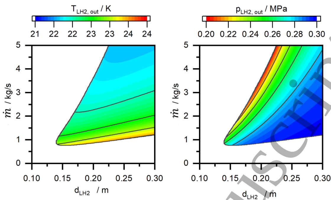
Figure 2: Outlet-temperature (left) and -pressure (right) of a HEP and the dependence on mass flow \dot{m} and LH 2 pipeline diameter d_{\text{LH}_2} (by project AppLHy!)
