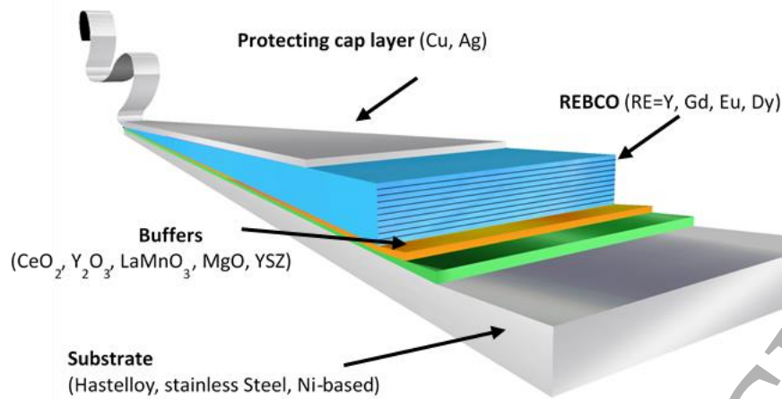
Figure 1. General schema of the coated conductor architecture. REBCO = \text{REBa}_2\text{Cu}_3\text{O}_7 , where RE is a Rare Earth or Yttrium.
