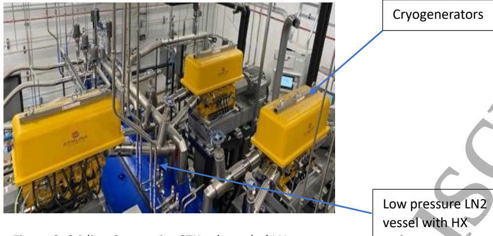
Figure 2: Stirling Cryogenics 67K sub-cooled LN 2 cable cooling system Courtesy ComEd and AMSC, USA
