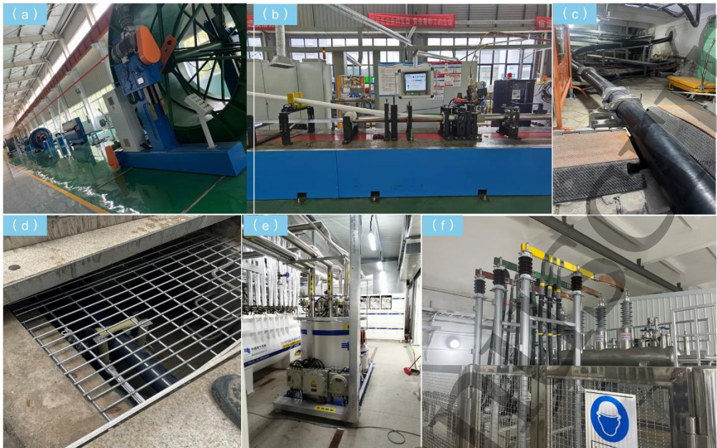
Figure 1. Landmark pictures of Shenzhen superconducting cable demonstration project. (a) Automated production line for concentric HTS cable cores. (b) Continuous welding and encapsulation production line for HTS cable core and cryogenic pipes. (c) Installed HTS cable in the cable tray. (d) Installed HTS cable in the cable trench. (e) Cryogenic refrigeration system. (f) HTS terminal in Binhe Substation.
