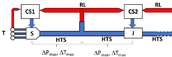
Figure 1b. Cooling principle for the SuperLink Project in Munich[7]. Legend: T (Terminations), S (splitterbox, where the three conductors were separated), J (cooling joint, where cooling liquid is returned from one side and injected from the other), CS1 (Cooling system at cable connection points), CS2 (intercooling system, second cooling system installed along the cable route), HTS (main serviceable cable length), RL (warm coolant return line).
