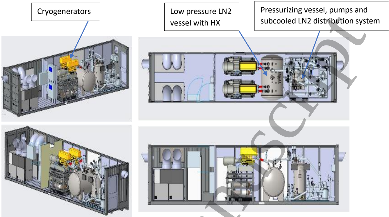
Figure 3: Stirling Cryogenics 67K sub-cooled containerized LN 2 cable cooling system Courtesy Supernode Ireland
