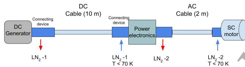
Figure 1: Schematic view of the ASCEND demonstrator. The links are cooled with flowing liquid nitrogen, the inlet and outlet of the cooling circuit is referred to as LN2-1 for the DC link, and LN2-2 for the AC Link.
