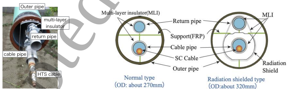
Cut model of the cryogenic pipe (normal type)
