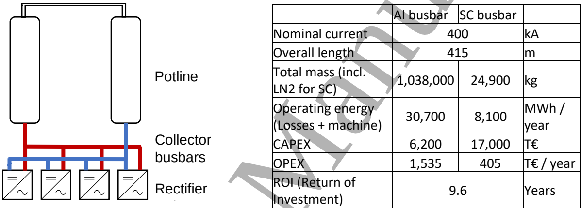
Figure 2: Comparison of equivalent aluminum and superconducting collector busbars for an aluminum cell room
