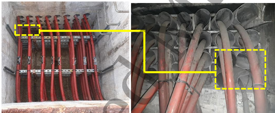
Figure 1. Saturated right of ways in railways infrastructure of big cities - Example at the Montparnasse Station in Paris with only few pipes left for future power increase only possible with superconducting cables.
