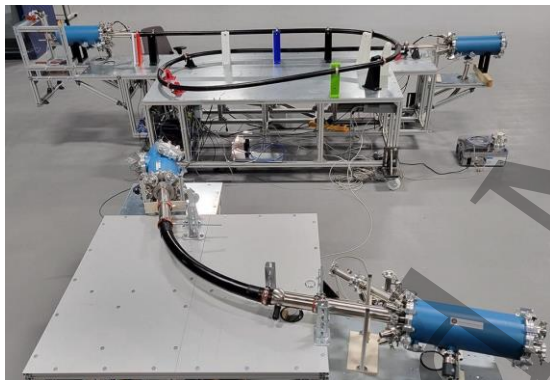
Figure 2: The superconducting DC (in the background) and the AC link (in the foreground) in Airbus Electric Aircraft Systems House, Ottobrunn during integration in the testbench in 2023.
