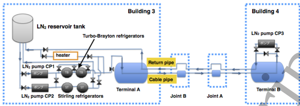
Figure 3. Schematic diagram for the cooling system
