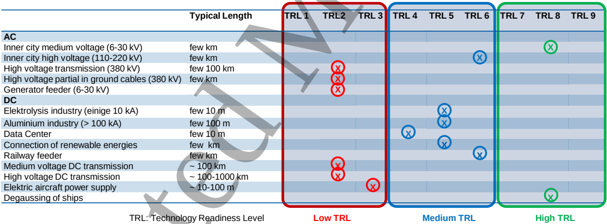
Figure 2. Technology readiness level (TRL) of several superconducting AC and DC cables and lines
