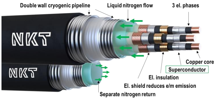
Figure 1a. Cable design for the SuperLink Project in Munich[7]
