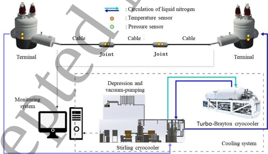
Figure 2. Schematics of the Shanghai 1.2 km long high-temperature superconducting cable and its auxiliary refrigeration and monitoring system.
