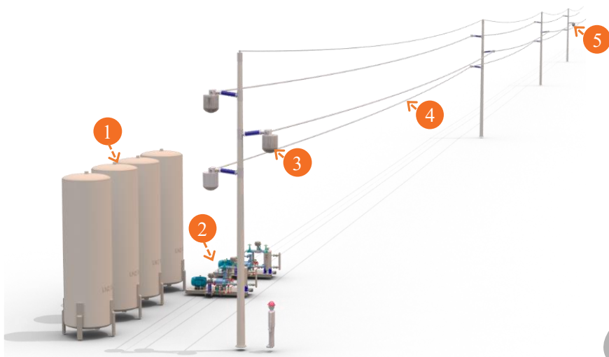
Figure 1. Shows anatomy of an O-SCTL solution with one phase of a three single-phase line pictured. 1) liquid nitrogen (LN2) generation/storage; 2) cryogenic conditioning infrastructure; 3) pole-top unit (terminal) 4) conductor assembly; 5) pole-top unit (heat exchanger).
