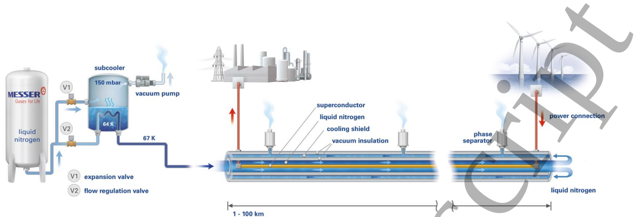
Figure 2. Cooling unit for a cable cryostat with active cooling shield
