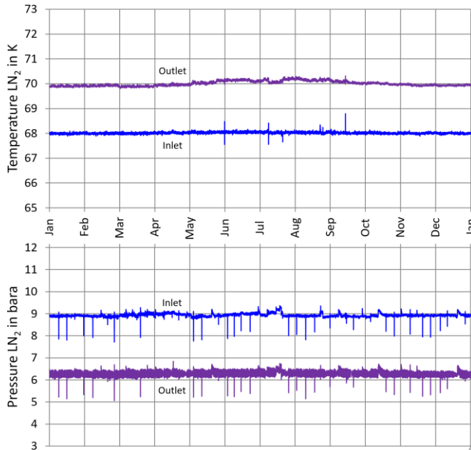
Fig. 2: Temperature and pressure history of the nitrogen supply during one year AmpaCity operation.
