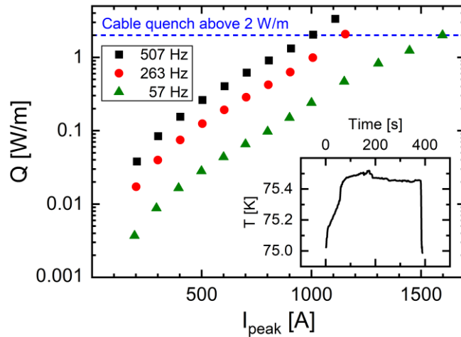
Figure 2. Ac loss of a 24-tape CORC® cable measured at 75 K in boiling liquid nitrogen as a function of peak current. The cable contained a 1 mm thick wrapped polyimide dielectric. Measurements were taken at frequencies of 57.3, 263, and 507 Hz. The dashed line indicates the loss of 2 W/m at which the cable would quench, independent of frequency. The inset shows the temperature as a function of time measured between the REBCO tapes and cable dielectric when operated at 507 Hz and a peak current of 998 A.
