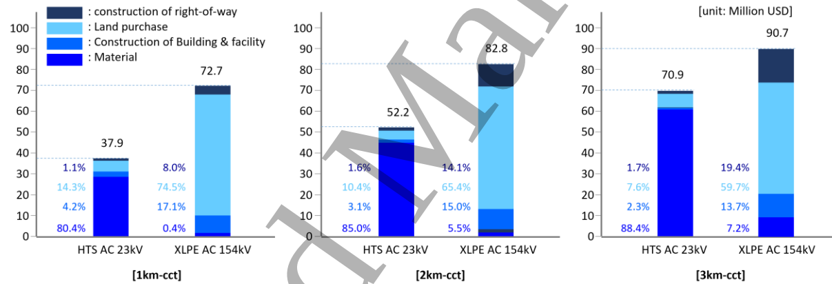
Figure 2: Comparative analysis on the economic feasibility between two solutions
