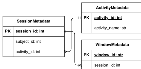
Figure 2: Entity-relationship diagram illustrating the metadata schema for the standardized data format.
