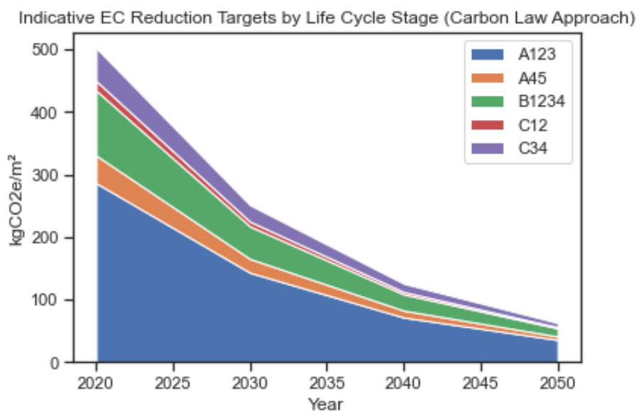
Figure 6. Indicative reduction targets for embodied carbon emission of both residential and non-residential buildings in different life cycle stages [kgCO 2 e/m 2 ], based on [11] and [12].
