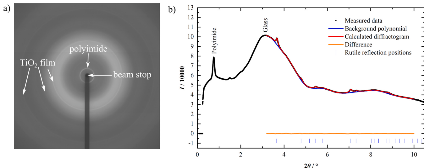
Fig. 11. Diffraction image of a 10 \mu\text{m} thick as-deposited \text{TiO}_2 PAD film on a soda-lime glass substrate as measured (a) and integrated by a 2D diffraction image (b). In (b) the integrated signal is shown in black. In addition, the data calculated by Rietveld refinement (red), as well as the background (blue) and the difference between calculated and measured data (orange) are shown.
