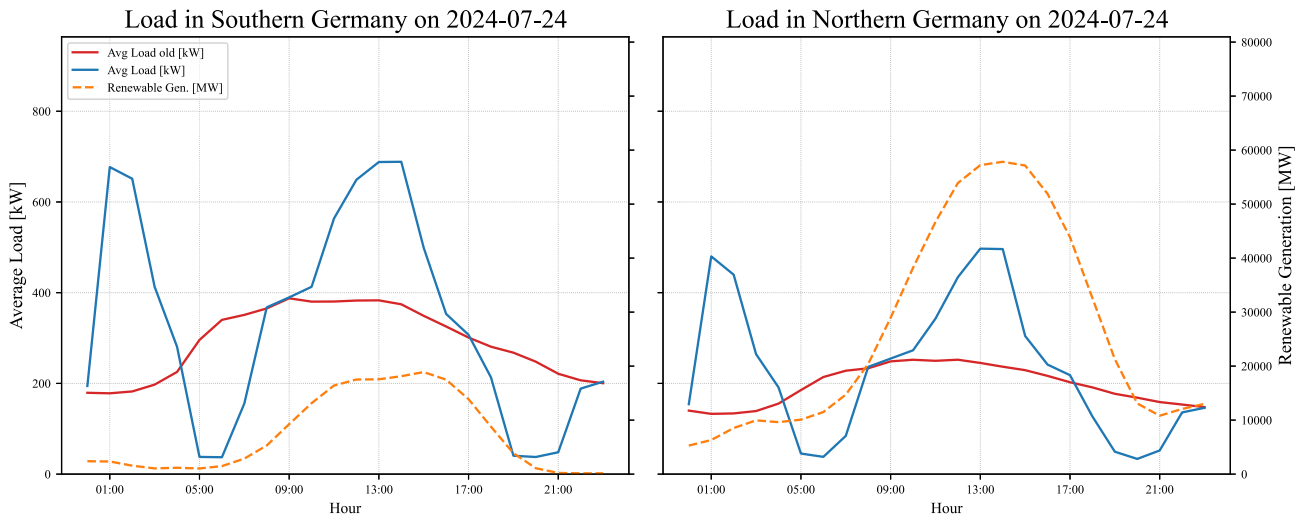
Fig. 6. Load change behavior in Northern and Southern Germany for Regulation 2.
