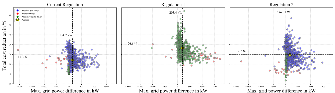
Fig. 3. Cost reduction potential compared to the change in grid power consumption.
