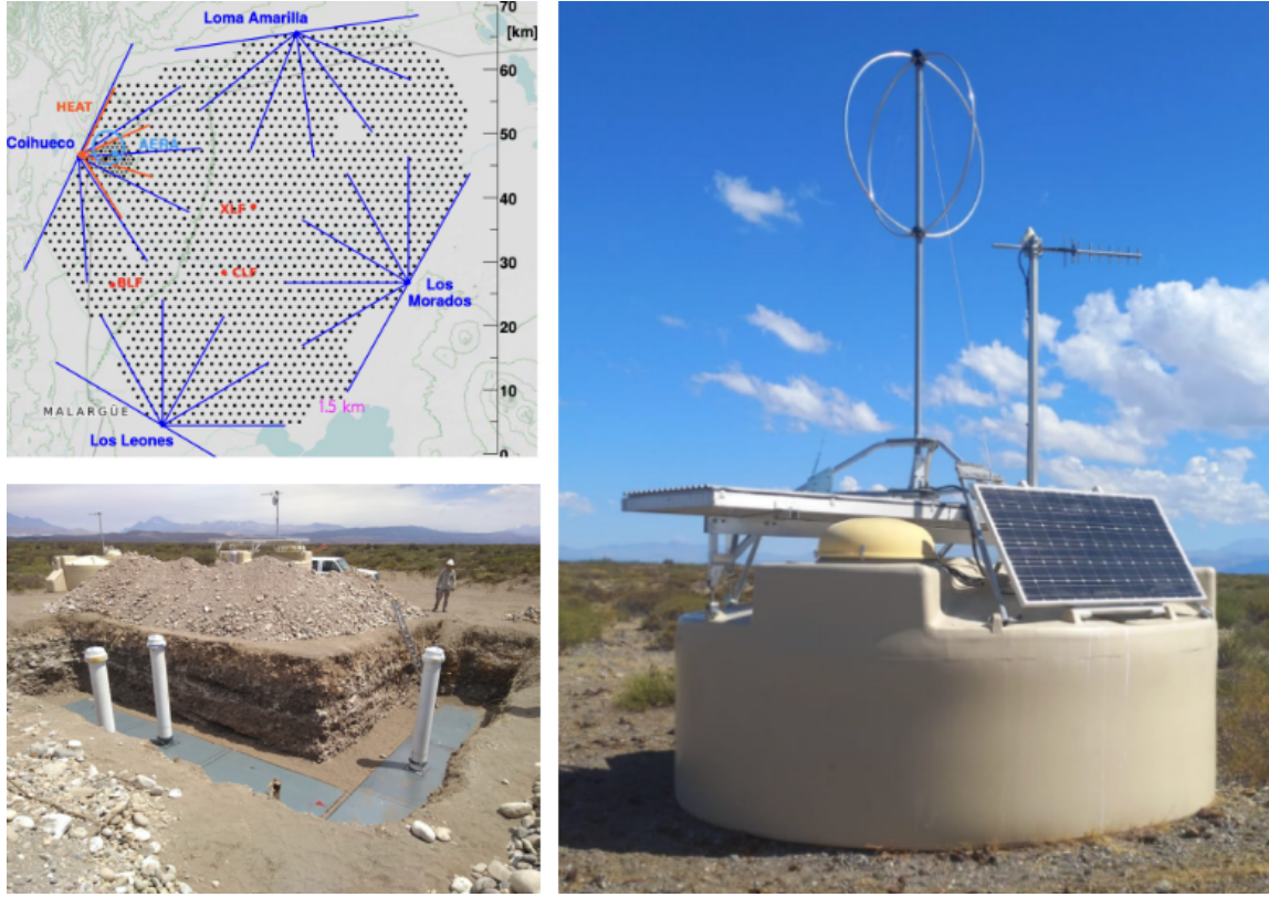
Figure 1: Top-left: layout of the Pierre Auger Observatory. Black dots represent surface detector stations and blue lines indicate the approximate field of view of the fluorescence telescopes in its four sites. The SD-750 and SD-433 arrays are located near the Coihueco site. Bottom-left: Underground Muon Detector station under deployment. Right: upgraded Water-Cherenkov detector, with a Scintillator detector and a Radio antenna.
