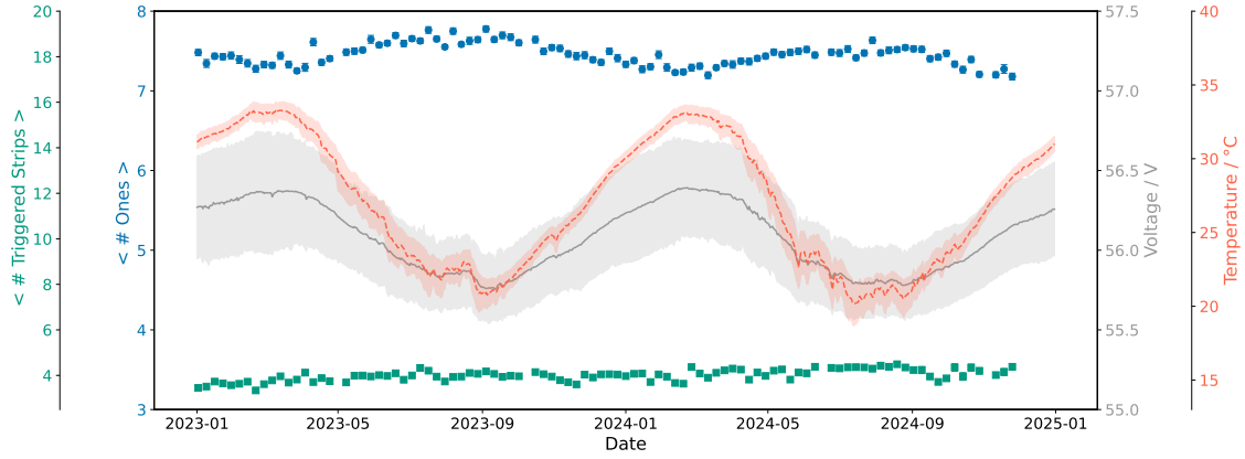
Figure 6: Daily averages of UMD monitoring parameters across all operational modules from 2023 to 2025: temperature measured at the high-voltage source (pink dashed line), applied voltage (gray solid line), average number of ones per trace (blue circles), and the average number of triggered strips per event with muon-like pattern (green squares).
