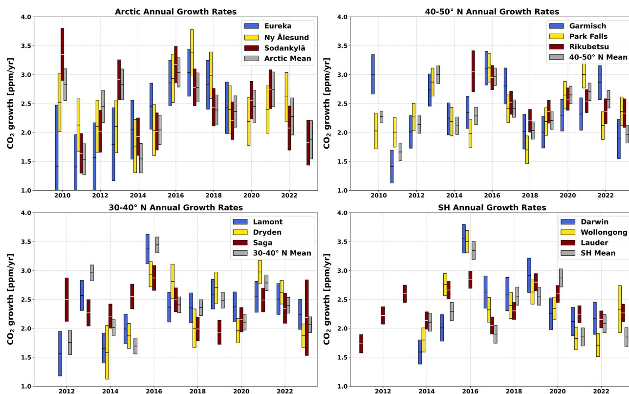
Figure A5. Annual CO 2 growth rates derived from TCCON stations, covering 2009–2024. Each panel corresponds to a different study region: (top left) Arctic sites, (top right) 40–50° N, (bottom left) 30–40° N, and (bottom right) Southern Hemisphere sites. Colored bars show annual growth rates for individual stations, and grey bars indicate the average of all sites within the region. The central line within each bar indicates the median growth rate, and the bar length reflects the associated uncertainty.
