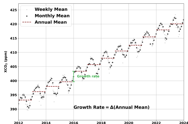
(a) Monthly Mean (MM)
