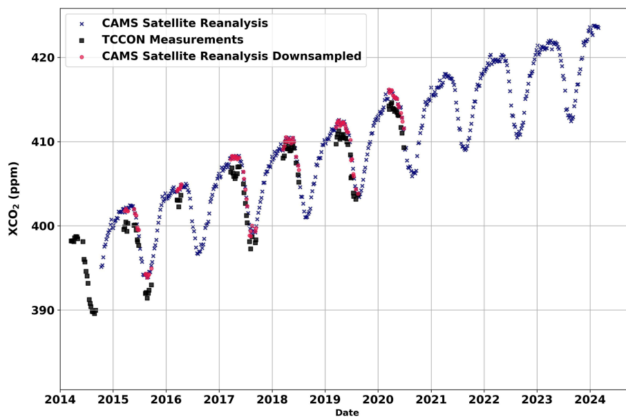
Figure A4. Time series of weekly averaged XCO 2 from the Eureka TCCON overlaid with CAMS reanalysis data from the nearest grid point to each as well as the downsampled CAMS timeseries.
