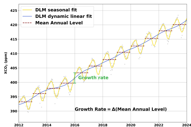
(c) Dynamic Linear Model (DLM)
