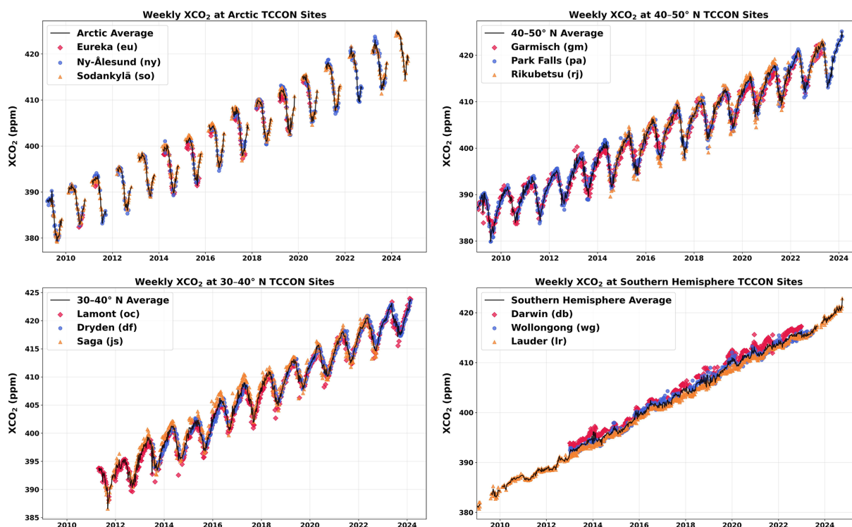
Figure A1. Time series of weekly XCO 2 measurements from selected TCCON stations and regional averages, covering the period from 2009 to 2024. Each panel corresponds to a different study region: (top left) Arctic sites, (top right) 40–50° N, (bottom left) 30–40° N, and (bottom right) Southern Hemisphere sites. Colored markers represent individual TCCON station measurements, while the black line shows the smoothed regional average, with gaps masked where data is not available.
