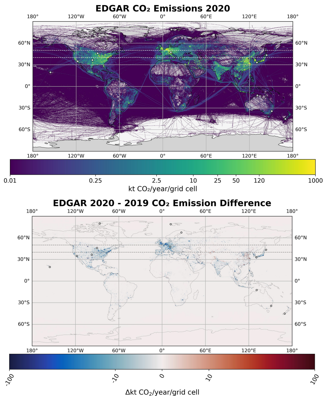
Figure A6. Top: Map of 2020 fossil fuel emissions based on the EDGAR 2020 fossil fuel flux data, displayed at a 0.1^\circ \times 0.1^\circ resolution (Crippa et al., 2023). Bottom: Map showing the difference in emissions between 2020 and 2019 at the same resolution. The locations of TCCON stations used in this study are marked with yellow circles, while additional horizontal lines at 40 and 50° N are added to indicate the latitude bands used for regional analysis. Global map based on Natural Earth public domain data and plotted using the Cartopy Python library (Met Office, 2024; Natural Earth, 2025).
