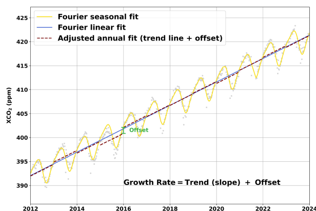
(b) Fourier Fit (FF)
