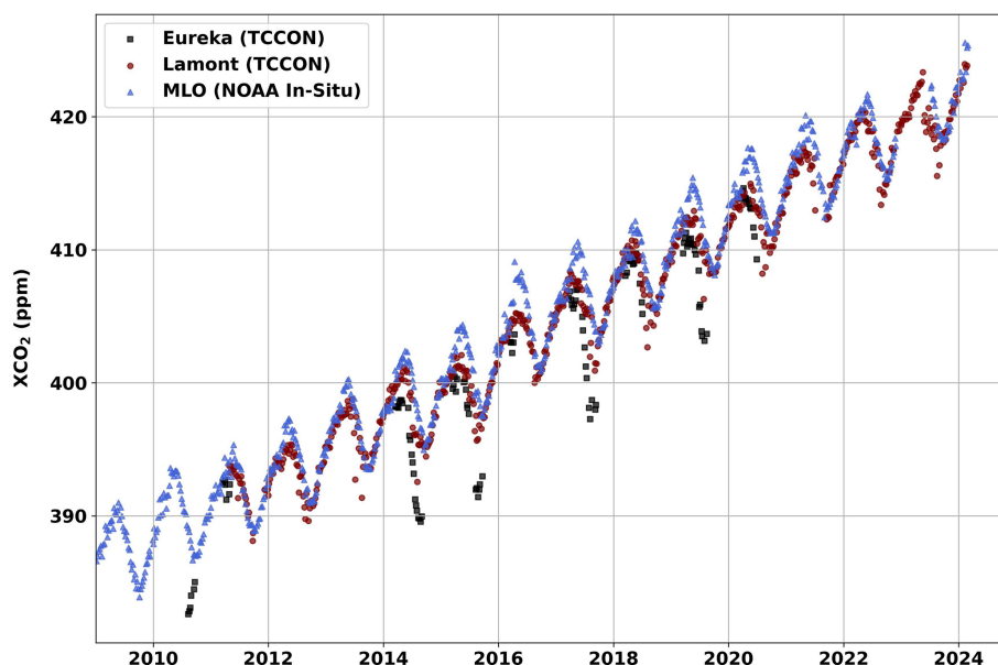
Figure A3. Time series of weekly averaged ground-level CO 2 concentrations from the NOAA MLO site and weekly averaged XCO 2 measurements from the Lamont and Eureka TCCON sites
