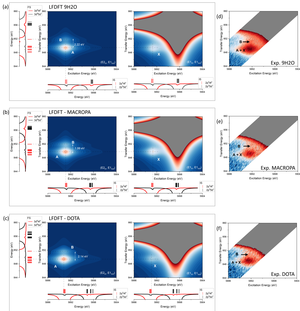
Figure 5. La L_2 -edge CC-RIXS of the complexes. (a) Calculated CC-RIXS map for 9H2O. (b) MACROPA and (c) DOTA. (d) Experimental CC-RIXS map for 9H2O. (e) MACROPA and (f) DOTA. Note that the pre-edge (PE) features with multiple signal A, B and X are highlighted for both calculated (LFDFT) and experimental (Exp.) data. In the calculated data, the calculated multiplet energies and ligand-field splitting of the IS and FS electronic states are also shown for discussion. These are obtained by using LFDFT with the PBE 31 DFT functional based on the optimized structures of 9H2O, MACROPA and DOTA obtained with the same functional (Supplementary Tables 2-7). The calculated maps result from two different mechanisms (see the text for details): ( E_{2in}, E_{1out} ) (left-side in each panel) and ( E_{1in}, E_{1out} ) (right-side). For each multiplet level ( i ), the sum of the squared of the configuration interaction coefficients ( c_i^2 ) over the Slater determinants that have 4f (in red) and 5d (in black) spin-orbitals are plotted, and show a diagnostic for the degree of mixing between 2p^5 4f^1 and 2p^5 5d^1 configurations in IS and between 3d^9 4f^1 and 3d^9 5d^1 configurations in the FS. To aid visualisation of the low-intensity PE features, the experimental CC-RIXS maps (d-f) are plotted on a logarithmic intensity scale. See also in the Supplementary Figure 6 and Supplementary Figure 7, selective cross sections of the experimental CC-RIXS maps are given.
