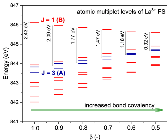
Figure 4. Nephelauxetic effects on the FS electronic structure. Changes of the atomic multiplet energy levels (red and blue bars) of 3d^9 4f^1 as function of the nephelauxetic ratio \beta showing the energy spacing between the J = 3 and J = 1 states that are responsible for the PE peaks A and B in the CC-RIXS map, respectively. Note that only the 3d^3_{3/2} 4f^1 energy levels are shown for clarity.
