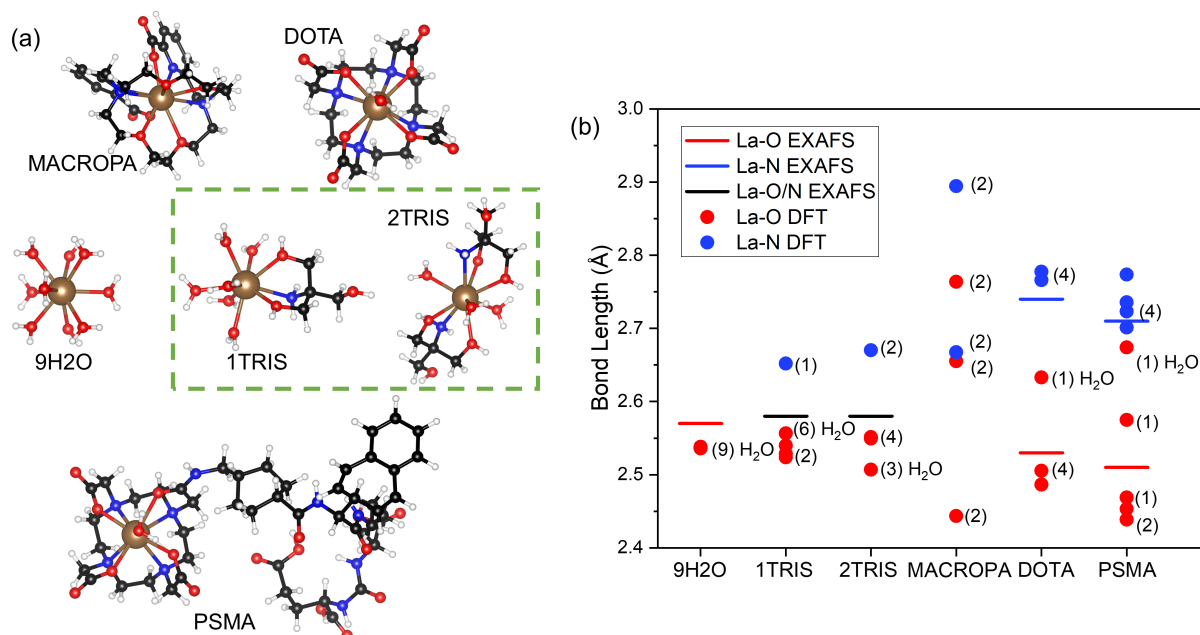
Figure 1. Atomic structures of the \text{La}^{3+} homologues for radiopharmaceuticals. (a) Ball-and-stick models for [\text{La}(\text{MACROPA})]^{1+} (MACROPA), [\text{La}(\text{DOTA})\text{H}_2\text{O}]^{1-} (DOTA), [\text{La}(\text{H}_2\text{O})_9]^{3+} (9H 2 O), [\text{La}(\text{TRIS})(\text{H}_2\text{O})_6]^{3+} (1TRIS), [\text{La}(\text{TRIS})_2(\text{H}_2\text{O})_3]^{3+} (2TRIS), and [\text{La}(\text{PSMA-617})\text{H}_2\text{O}] (PSMA). Color code: C (black), H (white), N (blue), O (red), La (brown). (b) Comparison between the experimentally derived (La L 3 -edge EXAFS) and theoretically calculated (DFT) La-O and La-N bond lengths. Details about the EXAFS analysis are available in the Supplementary Figure 1 and Supplementary Table 1. The presented theoretical bond lengths correspond to DFT results with the PBE0 31 functional (Supplementary Tables S2-S7). Note that the multiplicity of the La-ligand bonds are also depicted in brackets.
