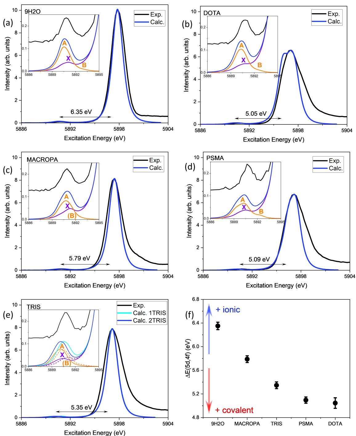
Figure 6. Calculated versus experimental La L_2 -edge HR-XANES. (a) 9H 2 O. (b) DOTA (b). (c) MACROPA. (d) PSMA. (e) TRIS. The experimental spectra are depicted in black. The calculated spectra are shown in blue and cyan. (f) Correlation between the complexes and the \Delta E(5d,4f) . Note that in (e) for TRIS, calculated spectra for 1TRIS (cyan) and 2TRIS (blue) are separately shown. Note also that in (a-e) the calculations are done using LFDFT with the PBE0 31 DFT functional based on the optimized structures obtained with the same functional (Supplementary Tables 2-7). In each panel, the experimental derived \Delta E(5d,4f) are shown for convenience. The HR-XANES spectra are obtained from cross-sections of the calculated CC-RIXS maps at the emission energy that corresponds to the maximum of WL. The insets show highlight of the pre-edge energy region of the spectra, showing also the individual contributions of the ( E_{1in} , E_{1out} ) (violet) and ( E_{2in} , E_{1out} ) (orange) mechanisms in the CC-RIXS process. For TRIS: 1TRIS (dashed line) and 2TRIS (solid line).
