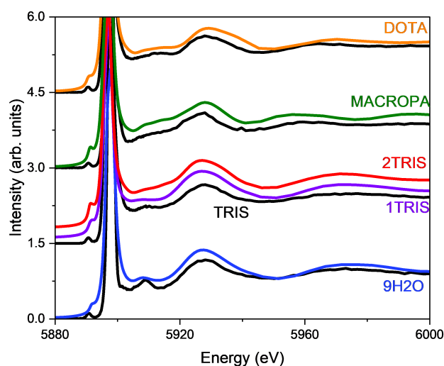
Figure 9. Post-edge La L 2 -edge HR-XANES analysis.
