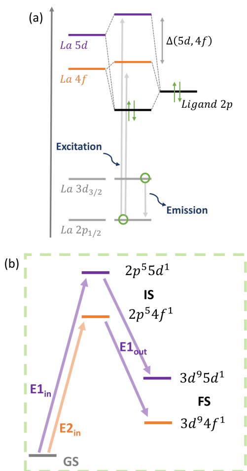
Figure 2. Mechanism of the La L_2 -edge CC-RIXS process. (a) Representation of two-photon processes whereby x-ray light is absorbed by exciting one electron from La core 2p_{1/2} shell. This is followed by relaxation, where electron in La core 3d orbitals fill the 2p core hole. (b) Electronic structures that results from the CC-RIXS mechanism: ground-state (GS) and excited intermediate-state (IS) and final-state (FS). Note that the electron transitions are governed by the selection rules of both the electric-dipole (E1) and electric-quadrupole (E2) transitions. The total CC-RIXS signal is given by |(E1_{in}+E2_{in})E1_{out}|^2 (see also the Supplementary Theoretical Model).
