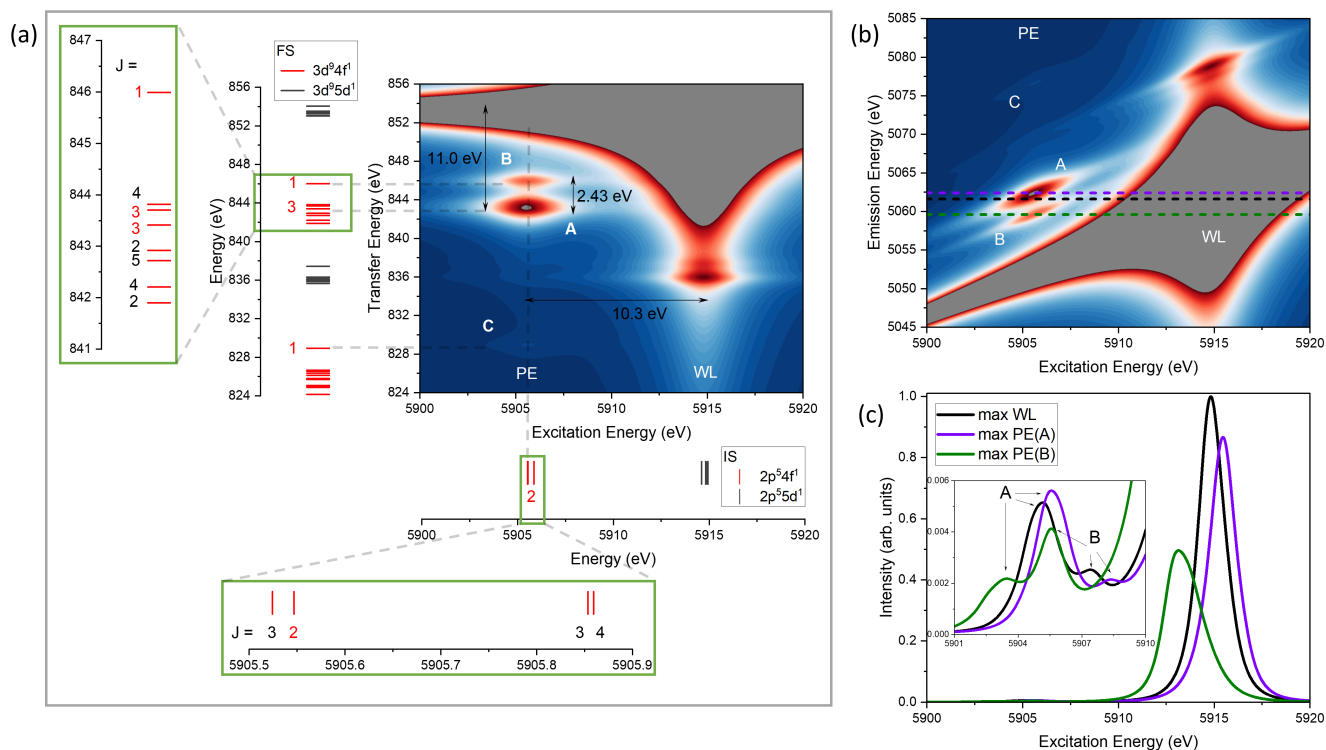
Figure 3. La L 2 -edge CC-RIXS of La 3+ free ion. (a) Calculated map (LFDFT) showing different features that correspond to the main absorption edge peak (WL) and the pre-edge (PE) A, B, and C signals, together with the calculated multiplet energies of the IS and FS electronic states (red and black bars) of the CC-RIXS process. (b) Translation of the calculated map with respect to the excitation and emission energies, showing also selected cross-sections (colored dashed lines) representing HR-XANES spectra. (c) Calculated HR-XANES spectral profiles for La L 2 -edge of La 3+ free ion following selective cross-sections. Note that in (a) the map is represented with respect to the excitation and transfer energies for direct comparison with the electronic structure. The calculations are done using LFDFT with the PBE0 31 DFT functional. Note also that the multiplet energy levels are characterized with their total angular momentum J values. The 2p 5 4f 1 (red bars) and 2p 5 5d 1 (black bars) configurations, relevant to IS, give rise to 1,3 D + 1,3 F + 1,3 G and 1,3 P + 1,3 D + 1,3 F atomic multiplet terms (Russel-Saunders coupling). When spin-orbit coupling is introduced, the terms split into total angular momentum J multiplets with J = 1 + 2 + 2 + 3 + 3 + 4 + 4 + 5 (2p 3/2 3 4f 1 ), J = 2 + 3 + 3 + 4 (2p 1/2 1 4f 1 ), J = 0 + 1 + 1 + 2 + 2 + 3 + 3 + 4 (2p 3/2 3 5d 1 ) and J = 1 + 2 + 2 + 3 (2p 1/2 1 5d 1 ). The 3d 9 4f 1 configuration (red bars), relevant to FS, gives rise to 1,3 P + 1,3 D + 1,3 F + 1,3 G + 1,3 H terms (Russel-Saunders coupling). With spin-orbit coupling, the terms split into J = 1 P 1 + 1 D 2 + 1 F 3 + 1 G 4 + 3 P 0,1,2 + 3 D 1,2,3 + 3 F 2,3,4 + 3 G 3,4,5 + 3 H 4,5,6 . Note that in (b) the cross-sections are selectively chosen along the emission energy that corresponds to the maximum of the WL (black dashed line) and PE peaks A (violet dashed line) and B (green dashed line).
