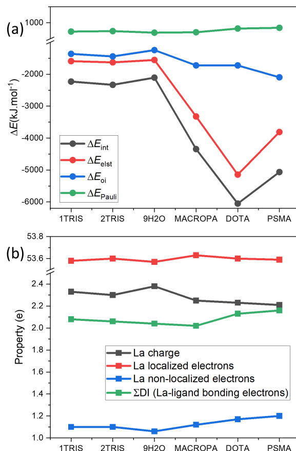
Figure 8. Ab initio Bond analysis. (a) Energy Decomposition Analysis (EDA). (b) Quantum Theory of Atom in Molecules (QTAIM) analysis. Different metrics that are used to describe chemical bonds are shown for 9H 2 O, 1TRIS, 2TRIS, MACROPA, DOTA and PSMA (see the Text for details). Note that the calculations are done using DFT with the TPSSH 88 DFT functional based on the optimized structures obtained with the same functional (Supplementary Tables 2-7). Description of the bond analysis metrics are available elsewhere. 85,87
