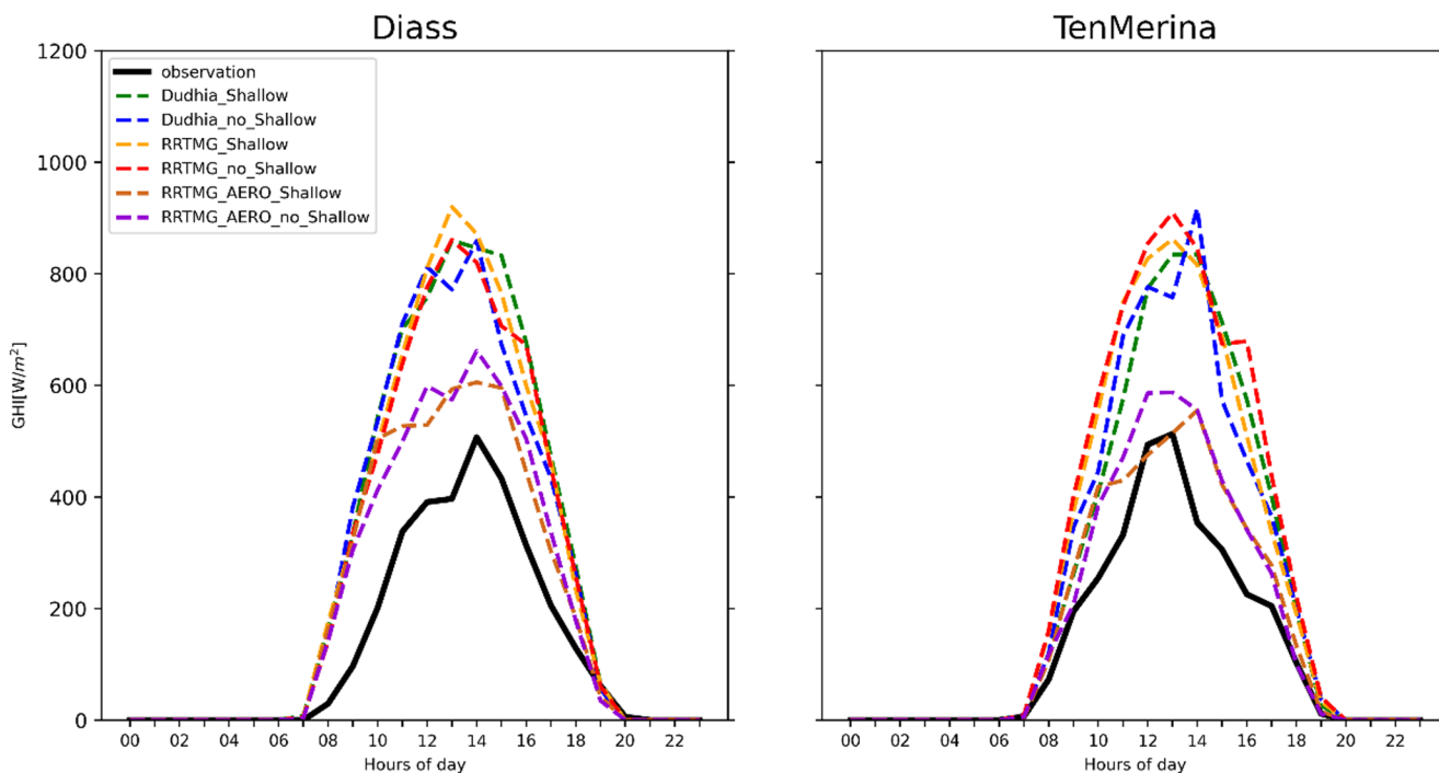
Fig. 7 Yearly average diurnal cycle of observed GHI at the two stations, along with simulated GHI from different WRF Solar experiments under cloudy-sky conditions
