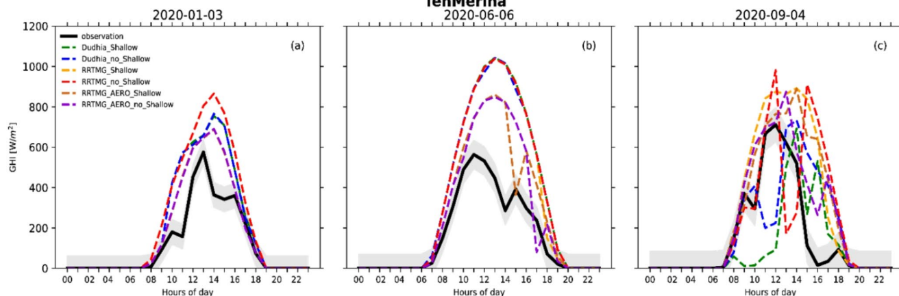
Fig. 11 Diurnal variation of GHI for the WRF-Solar configurations and observations at the two stations under cloudy-sky conditions
