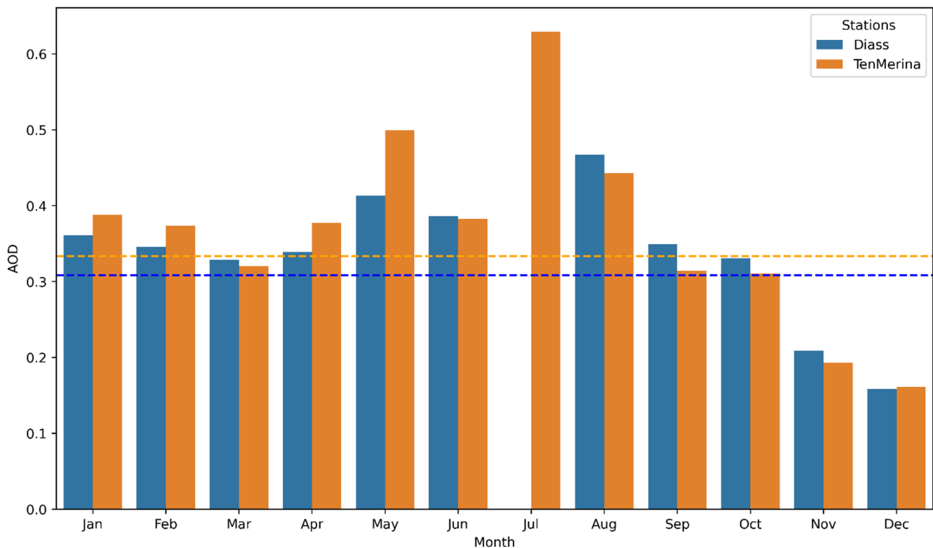
Fig. 6 Monthly AOD distribution over Ten Merina and Diass for 2020 under clear-sky conditions. The dashed orange and blue lines indicate the mean of the AOD in the two stations
