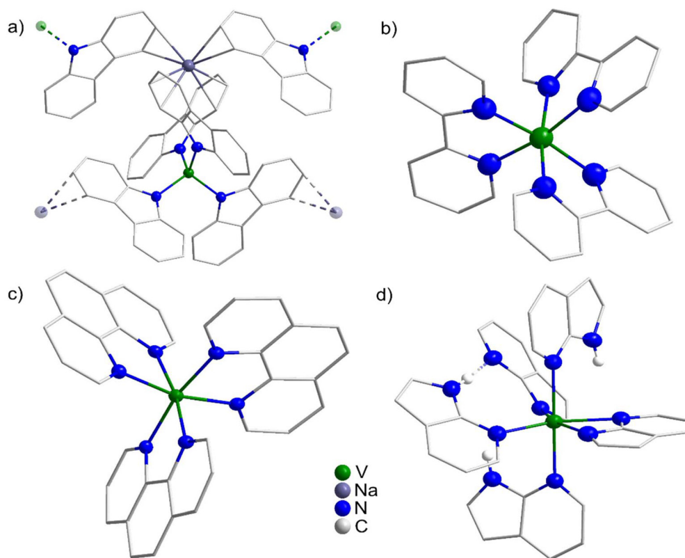
Fig. 4 Molecular structures of vanadium compounds with N-heterocycles: (a) [NaV(Cbz) 4 ] ( 1 ), (b) [V(bipy) 3 ] ( 2 ), (c) [V(phen) 3 ] ( 3 ), and (d) [V(η 1 -Hai) 3 (η 2 -ai)(η 1 -ai)]-0.5 tol ( 4 ).
