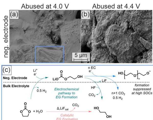
Fig. 3 Post-mortem SEM images of the negative electrode after thermal abuse containing 300 ppm \text{D}_2\text{O} at different OCPs and suggested mechanism for polymer formation. (a) Negative electrode after thermal abuse of cells with 300 ppm \text{D}_2\text{O} and an OCP of 4.0 V. (b) Negative electrode after thermal abuse with 300 ppm \text{D}_2\text{O} and an OCP of 4.4 V. (c) Reaction scheme of the polymerization processes triggered by formation (green route) 18,47 or during thermal abuse (orange route).
