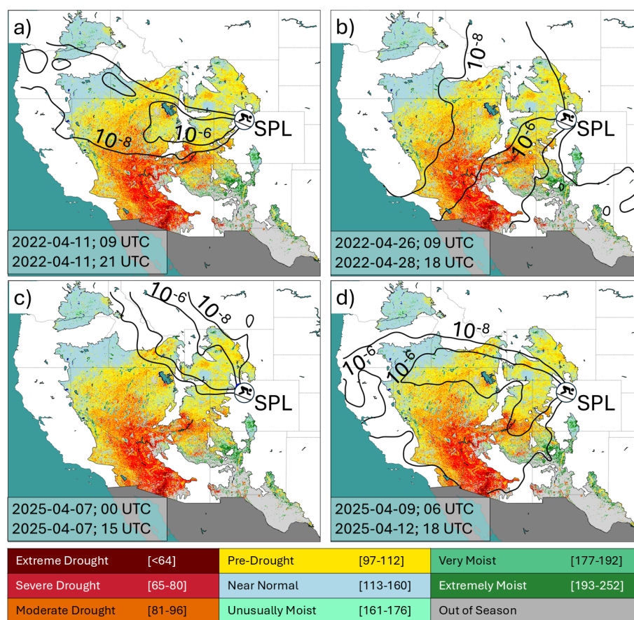
Figure 7. Footprints computed with the STILT model combined with surface maps of aridity using VegDRI of North American Desert ecoregions. Contours of the footprint are in units of \text{PPM}/\mu\text{mole m}^{-2} \text{s}^{-1} (surface influence footprint; Fasoli et al., 2018). Events of elevated INP concentrations were analyzed on the 11 April 2022 (a, INP concentration at -30^\circ\text{C} up to 1000 \text{ INP stdL}^{-1} ), on the 26 to 28 April 2022 (b, INP concentration at -30^\circ\text{C} up to 1000 \text{ INP stdL}^{-1} ), on the 7 April 2025 (c, INP concentration at -30^\circ\text{C} up to 500 \text{ INP stdL}^{-1} ), and on the 9 to 12 April 2025 (d, INP concentration at -30^\circ\text{C} up to 1000 \text{ INP stdL}^{-1} ).
