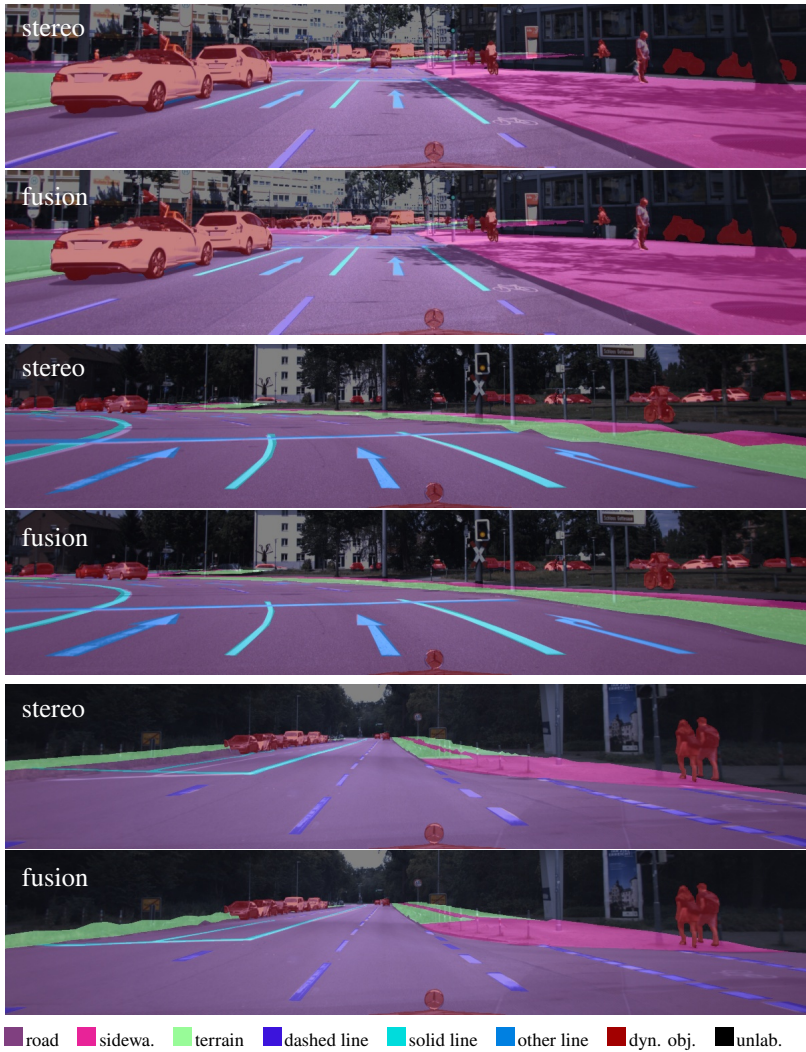
Figure 5.11: Qualitative evaluation of the dense surface feature map M_{DS} in three scenarios, comparing different reconstruction approaches. In each pair, the top image shows the stereo-based result, and the bottom image shows the fusion-based result. Areas in red are identified as occluded by dynamic objects, further described in Section 7.2.1. While both methods produce comparable reconstructions in the central region, the fusion-based approach provides greater accuracy near the boundaries of the field of view.
