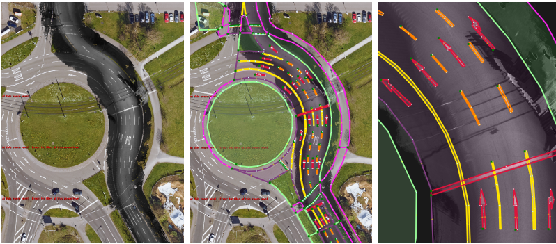
Figure 5.4: Annotation process of dense road surface features. Left: overlay of reconstructed road surface and aerial imagery, middle shows the annotated road surface features and right shows the same features in a zoomed-in view. The color coding is explained in Table A.3. Imagery: ©Stadt Karlsruhe | Liegenschaftsamt.
