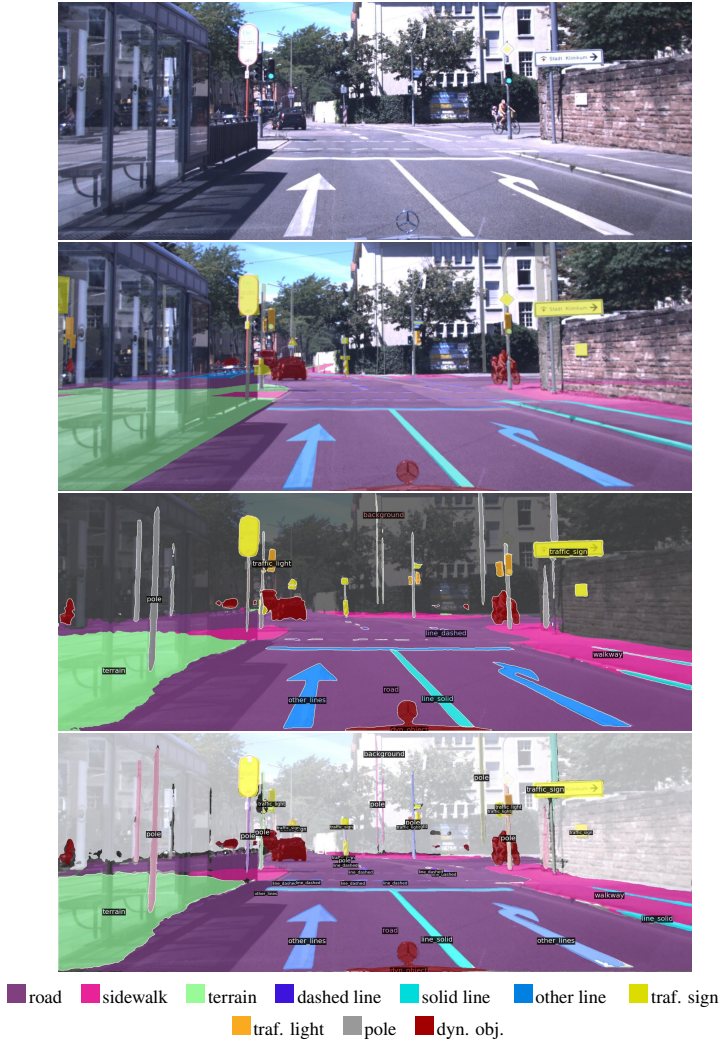
Figure 7.7: Qualitative evaluation of perspective panoptic segmentation. Top to bottom: RGB image, annotated ground truth, prediction results of panoptic segmentation shown as semantic masks and full panoptic output. Examples are from the geographically distinct test set.
