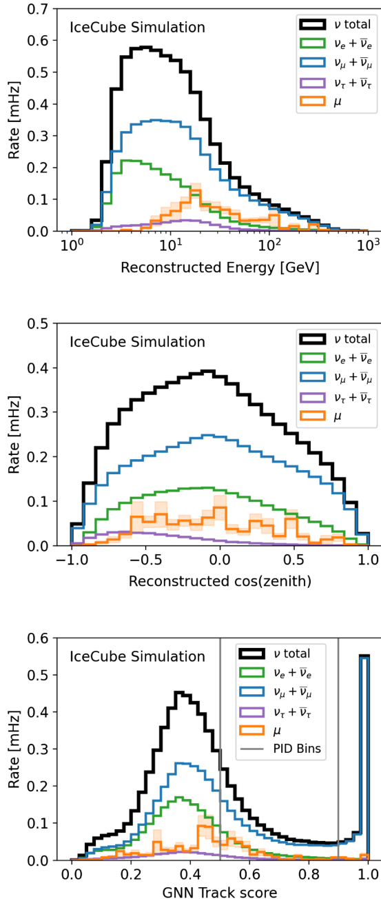
FIG. 7. Expected event distributions by flavor for the three variables used to bin events in the analysis: energy (top), \cos(\theta_{zen}) (middle), and particle identification score (bottom). In the bottom panel, a value of 1 indicates more tracklike events and the gray lines correspond to the boundaries used for particle classification.
