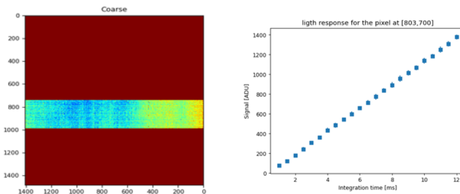
Figure 5. (left) ROI image of a dark sensor. (right) Using ROI settings that enable 1 kHz frame rate, integration time scan of steadily illuminated sensor provides a first sanity check.
