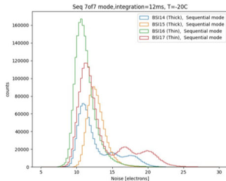
Figure 3. Comparison of baseline-operation (83 Hz, sequential 25/125 MHz) noise of 4 respin BSI sensors. Distinct contributions for some sensors are apparent — they are linked to ADC rows digitizing one of 7 rows within each row group (7 consecutive rows being read out simultaneously, before the rolling shutter continues to the next group of 7).
