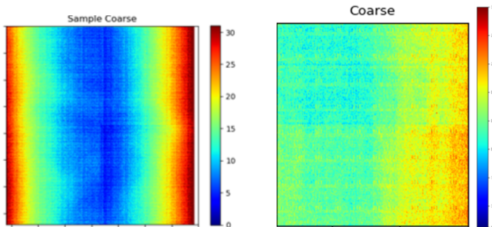
Figure 2. (left) Coarse ADC counts from a pre-respin sensor (BSI04) under experiment biasing conditions. While the central region of the dark image shows coarse values around 10 (and headroom to digitize signal at high amplification and correspondingly low noise), the edges already approach the maximum value 31. (right) The same image from a respin sensor (BSI14). While on one edge of the sensor some smaller form of the “bathtub”’s wall remains, on the opposite edge the effect is no longer apparent.
