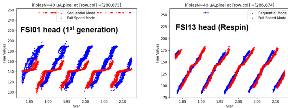
Figure 1. (left) ADC fine count ramps from a 1st generation sensor in full-speed (red) and sequential (blue) modes. (right) The same ADC fine count ramps, recorded with a 2nd generation “respin” sensor. The large plateau in the old chip’s full-speed operation is largely suppressed when the less parallellized (slower) sequential mode is used. Both ramps are significantly improved in the respin sensor; small differences between sequential and full-speed mode remain.
