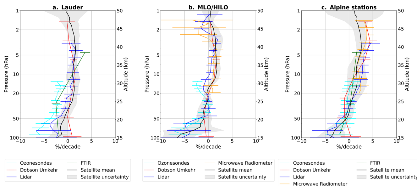
Figure 6. Ozone trend profiles (% per decade) for 2000 to 2024 at selected NDACC locations: (a) Lauder (New Zealand); (b) Mauna Loa and Hilo (Hawaii, USA); (c) Alpine stations that include (1) ozonesondes from Hohenpeißenberg, Payerne, and Haute Provence; (2) lidars from Hohenpeißenberg and Haute Provence; (3) Umkehr from Arosa and Haute Provence; (4) FTIR from Zugspitze and Jungfrauoch; (5) MWR in Payerne and Bern. Trend profiles are shown for ozonesondes (light blue), Dobson Umkehrs (red), lidars (dark blue), microwave radiometers (orange), and FTIR (green). For lidars, microwave radiometers and ozonesondes error bars are plotted every 2nd step for clarity. Also shown is the mean satellite trend profile, estimated by averaging MEGRIDOP, SWOOSH, SCIAMACHY-OMPS, and SBUV-MOD satellite data from the nearest grid boxes. Error bars represent the 95 % confidence intervals.
