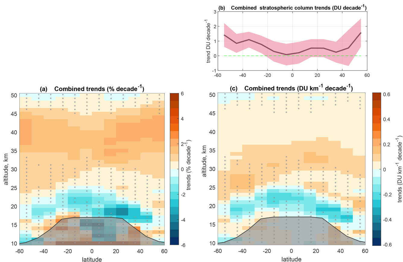
Figure 3. The combined (mean) ozone trends from eight merged satellite datasets as a function of latitude and altitude, expressed in % per decade (a) and DU km -1 per decade (c). The black lines show the climatological mean tropopause height. Gray stippling denotes results that are not significant at the 2σ level. (b) stratospheric column averaged trend (DU per decade), red line, with 2σ uncertainty (pink shading). The green dashed line in panel (b) highlights zero level.
