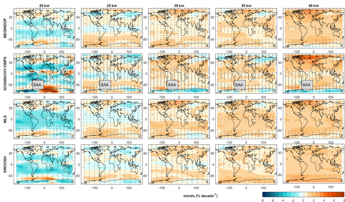
Figure 7. Latitude- and longitude-dependent ozone trends (% per decade) derived for the period 2003–2024 for five different altitude levels, based on the extended MEGRIDOP, SCIAMACHY-OMPS, SWOOSH, and MLS datasets. Gray dots indicate regions where the trends are not statistically significant at the 2\sigma level. For the SCIAMACHY-OMPS dataset, ozone trends in the Southern Atlantic Anomaly (SAA) region are not shown because SCIAMACHY data are flagged in this region.
