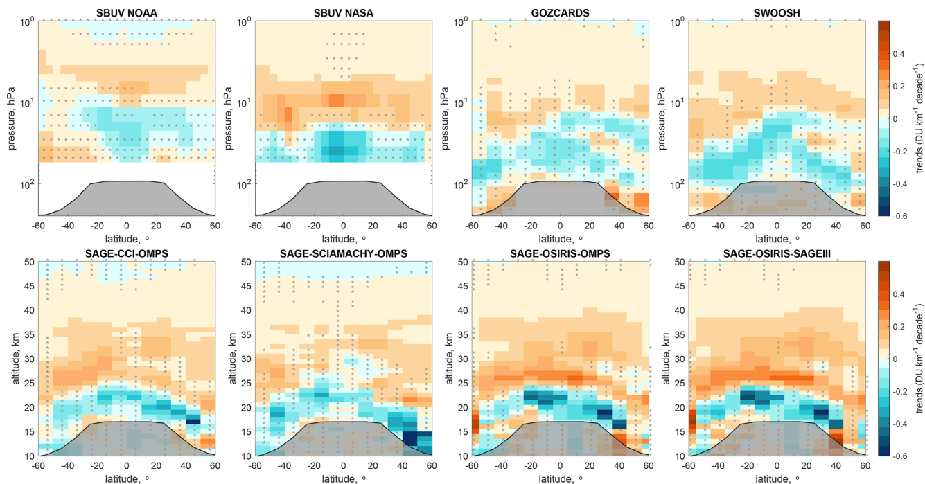
Figure 2. Same as Fig. 1, but trends are expressed in \text{DU km}^{-1} per decade.
