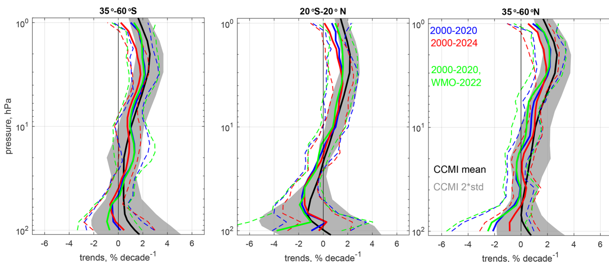
Figure 5. Comparison of simulated and observed post-2000 ozone trend profiles for the latitude bands 35–60° S (left panel), 20° S–20° N (center panel), and 35–60° N (right panel). Observed trends for the period 2000–2020 from GB22 and WMO-2022 are shown in green and the results with the updated regression model and updated datasets for the period from 2000 to 2020 and to 2024 are shown in blue and red, respectively. The mean model trends (CCMI REF-D2, 9 models) for 2000–2024 are shown in black with the 2\sigma uncertainties shown as shaded grey areas.
