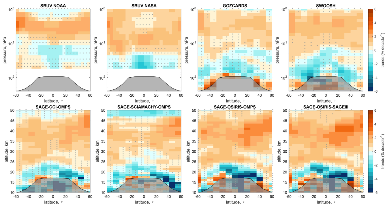
Figure 1. Ozone trends (% per decade) for the period 2000–2024 estimated from eight merged satellite data records using an independent linear trend model. Trends are shown for the SBUV COH (NOAA), SBUV MOD (NASA), SWOOSH, GOZCARDS, SAGE-CCI-OMPS, SAGE-SCIAMACHY-OMPS, SAGE-OSIRIS-OMPS, and SAGEII-OSIRIS-SAGEIII datasets. Gray stippling denotes results that are not significant at the 2\sigma level. Data are presented on the vertical coordinates (left-hand axis) and latitudinal grid associated with each dataset. The black lines show the mean climatological thermal tropopause height (or pressure) from the ERA-5 reanalysis. The trends in the upper troposphere are shaded and not assessed in this study.
