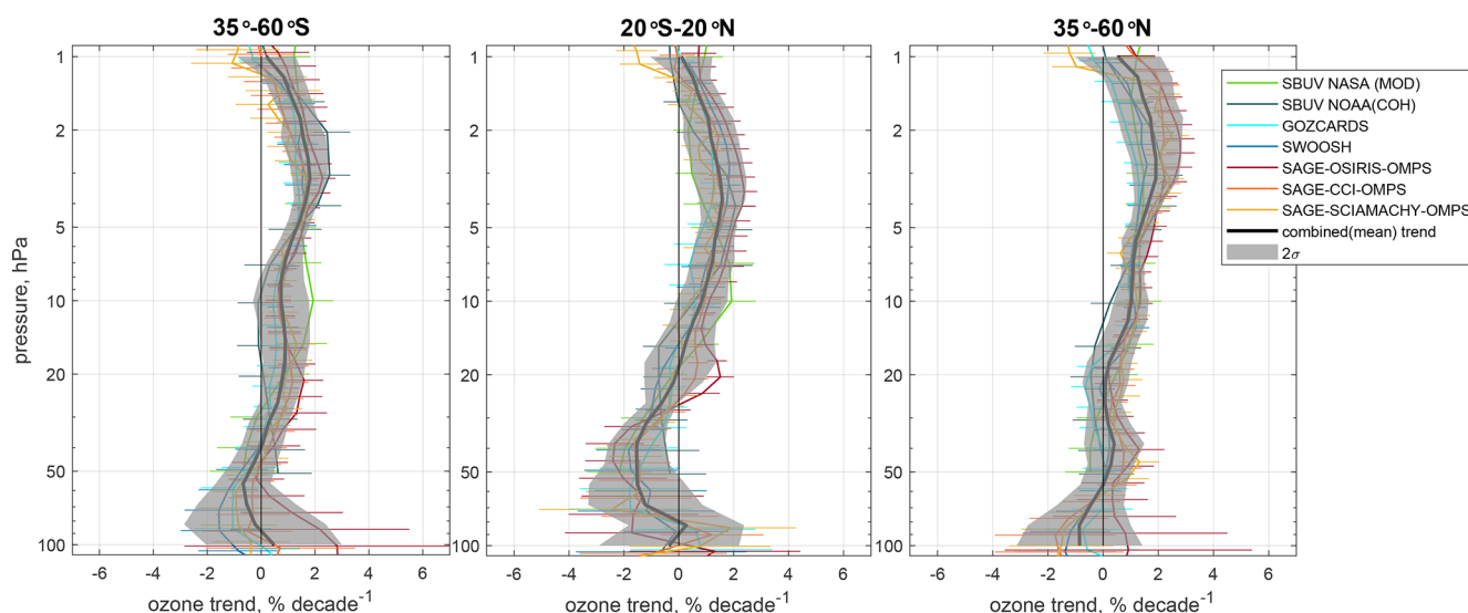
Figure 4. Ozone profile trends with 2\sigma uncertainties for the period 2000–2024 for latitude bands 35–60° S (left panel), 20° S–20° N (center panel), and 35–60° N (right panel). Colored lines are the trend estimates from seven individual merged datasets on their original vertical grids (SBUV NASA (MOD), SBUV NOAA (COH), GOZCARDS, SWOOSH, SAGE-OSIRIS-OMPS, SAGECCI-OMPS, and SAGE-SCIAMACHY-OMPS). Black lines represent the mean (combined) trends and gray shading indicates the 2\sigma uncertainty intervals for the combined trends.
