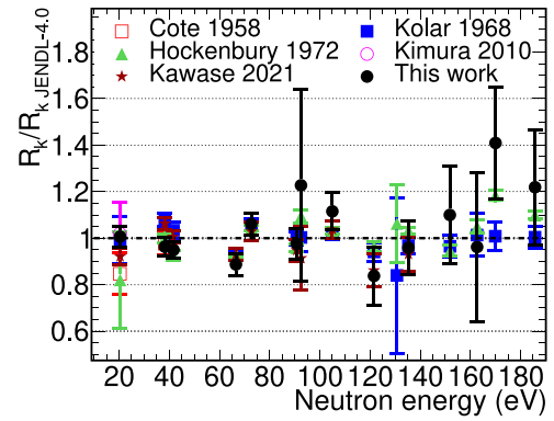
Fig. 8. Ratio between the ^{240}\text{Pu} R_k obtained in different experiments in the range from 20 to 190 eV, including this work, and JENDL-4.0.
