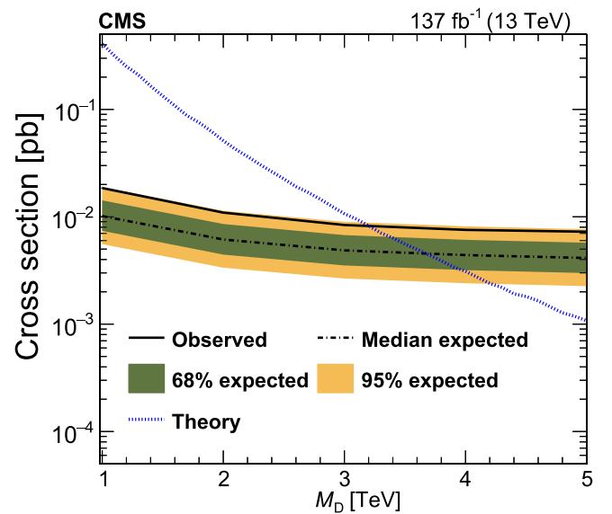
FIG. 10. The 95% CL upper limits on the ADD graviton production cross section as a function of M_{\text{D}} , for n = 3 extra dimensions.
