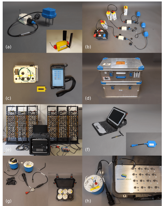
Figure 3 Large-N instrumentation, data exchange and processing equipment, and SmartSolo equipment. (a) Geospace 5 Hz 3C Land Cartesian GS-One LF geophone and GSB-3 seismic recorder. The inset shows the GSX3-LTE (renamed to GSX3-C) recorder with cellular network access. (b) Three acquisition configurations with one (top) or two (center, bottom) external battery solutions. (c) From left to right, source decoder, line health recorder, and tablet PC with line health viewer app. (d) Storage and transportation boxes for 16 GSB recorders (top) and 16 geophones (bottom). (e) Downloading, charging, and configuration racks for 6 \times 4 \times 12 = 288 GSB recorders. The unit in the front contains the Geospace GeoRes-XTC system manager server. (f) Laptop field server with line health data receiver in the inset. (g) Clockwise from the upper left: SmartSolo three-component 5 Hz geophone with black Single Port Dedicated All-In-One (AIO) data exchange unit, 5 Hz geophone without the AIO unit, magnet to switch the units on and off, connector, power plug, storage and transportation box in the inset. (h) Geophone connected to one of 16 slots in the battery charging box.
