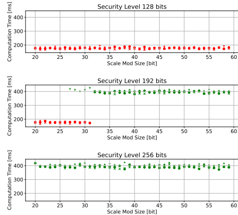
Figure 3: Computation time for the Multiplicative Function.
