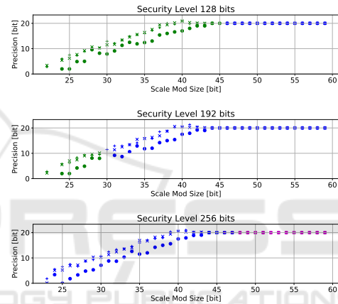
Figure 9: Precision for the Standard Deviation.
