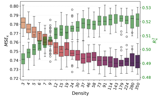
FIGURE 13. MSE and R^2 for the X-axis (steel).
