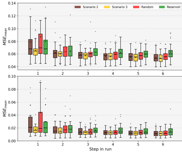
FIGURE 33. Comparison of scenario 2 and 3 with random sub-sampling and reservoir sampling for the DMC 60H (top) and the CMX 600V (bottom).
