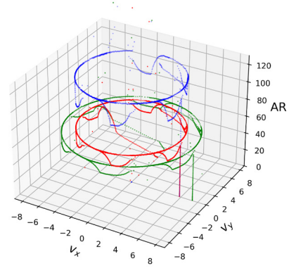
FIGURE 4. Gear part in the reduced feature representation at various feed velocities and cutting depths.
