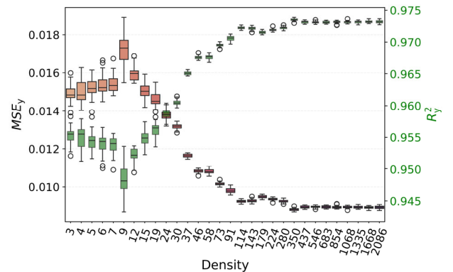
FIGURE 34. MSE and R^2 for the Y-axis (aluminum).
