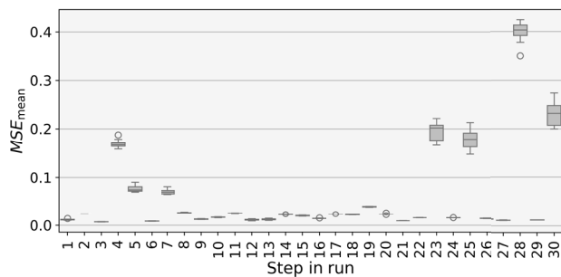
FIGURE 27. Results over all 30 runs of scenario 1 on the CMX 600V.
