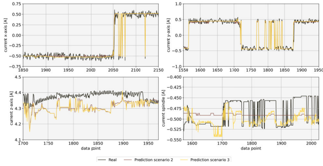
FIGURE 29. Prediction quality of scenario 2 and 3 in direct comparison.
