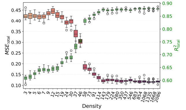
FIGURE 14. MSE_{total} and R^2_{total} different densities (aluminum).
