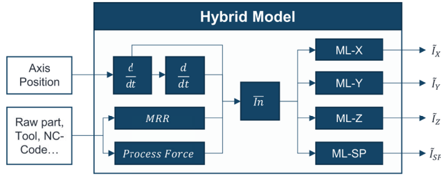
FIGURE 3. Hybrid model structure for reference signal prediction [3].
