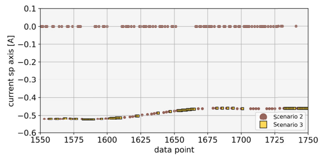
FIGURE 28. Training data spindle signal of scenario 2 and 3 for impeller 8.
