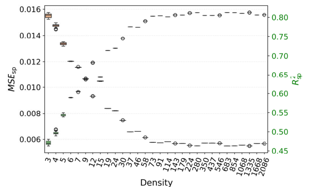
FIGURE 35. MSE and R^2 for the SP-axis (aluminum).
