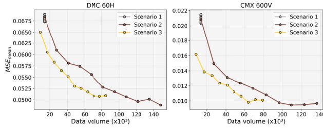
FIGURE 30. Median MSE_{\text{mean}} as a function of data volume.
