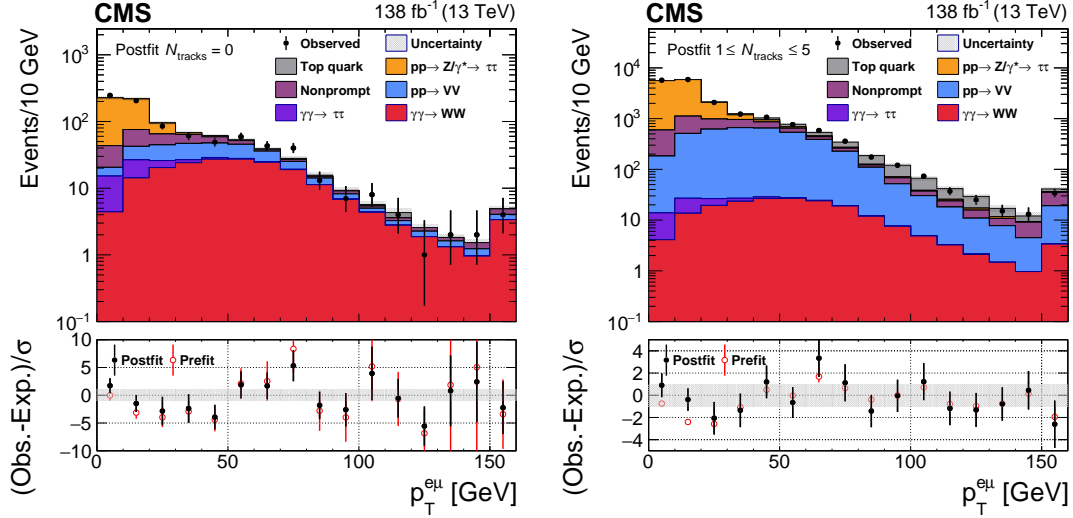
Figure 2: Observed and predicted p_T^{e\mu} distributions for events with N_{\text{tracks}} = 0 (SR, left) or 1 \leq N_{\text{tracks}} \leq 5 (CR, right), using 2016–2018 data. The distributions are shown after the maximum likelihood fit to the data (“postfit distributions”). The observed data and their associated Poissonian statistical uncertainty are shown with black markers with vertical error bars. The uncertainty band accounts for all sources of background and signal uncertainty, systematic as well as statistical, after the fit. The last bin includes the overflow. The lower panels show the ratio of data to sum of signal and background contributions, before (prefit, open red circles) and after (black full markers) the maximum likelihood fit.
