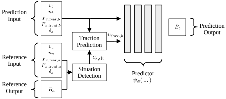
Figure 4.16: Illustration of the drivetrain prediction model with corresponding variables.
