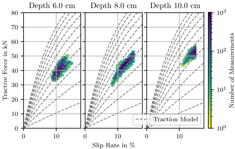
Figure 5.20: Transfer experiments: Traction measurements.
