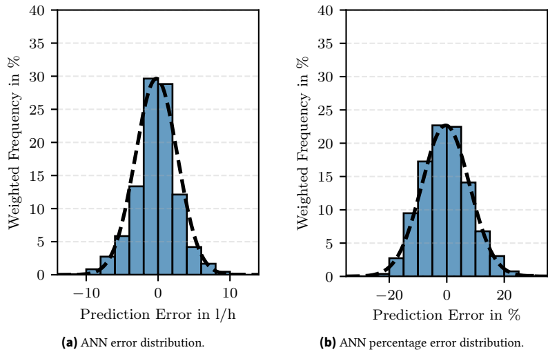
Figure A.2: Main experiment: ANN-based process load model combined with drivetrain model fuel rate prediction error histograms.
