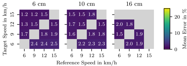
Figure 5.13: Drivetrain model: Fuel rate prediction error for different working depths.
