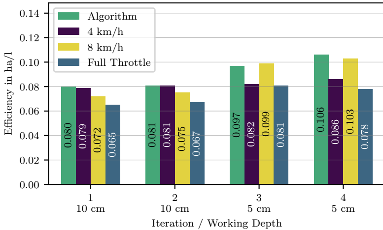
Figure 5.23: Optimization results: Average efficiency of the algorithm compared to static control inputs in parallel lanes across four experimental iterations, two with 10 cm working depth and two with 5 cm working depth.
