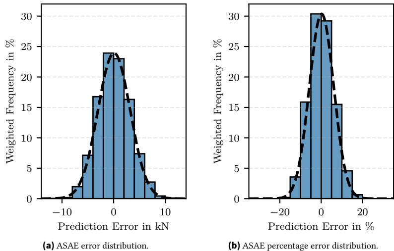
Figure A.3: Process load transferability experiment: ASAE model draft force prediction error histograms.
