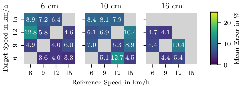
Figure 5.15: ANN model combined with drivetrain model: Fuel rate prediction error for different working depths.
