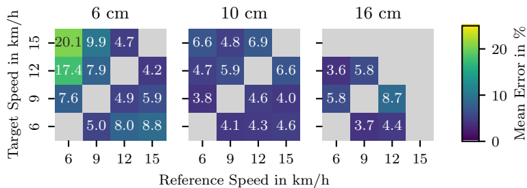
Figure 5.14: ASAE model combined with drivetrain model: Fuel rate prediction error for different working depths.
