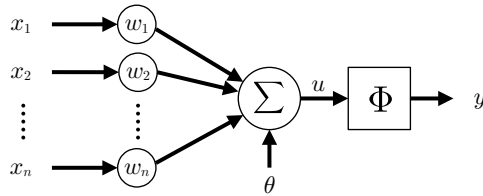
Figure 2.2: Visualization of an artificial neuron (inspired by [60]).
