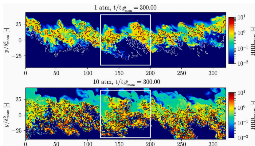
Fig. 9. Normalized heat release rate at the same normalized time (Adapt from Ref. [92] with permission).
