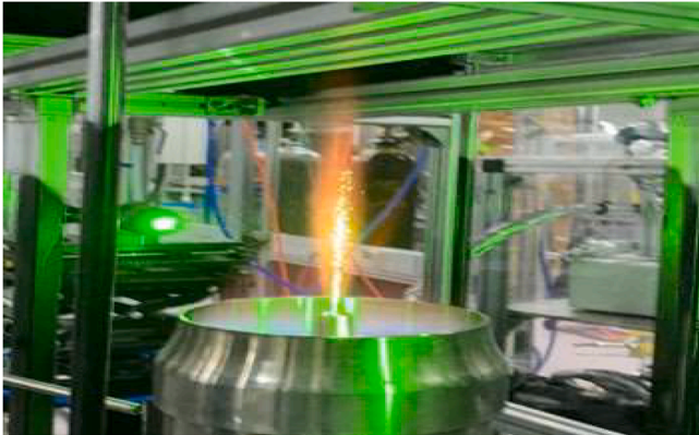
Fig. 15. Digital image of the liquid ammonia jet from experiments using MIE scattering (Reprint from Ref. [127] with permission).
