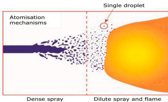
Fig. 11. Schematic representation of liquid fuel spray combustion (Reprint from Ref. [109] with permission).
