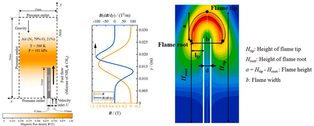
Fig. 6. Computational domain (left), boundary conditions(center) and schematic of laminar micro-diffusion flame configuration (right). (Reprint from Ref. [52]) with permission).
