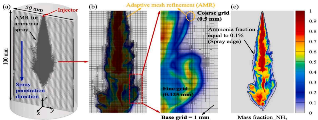
Fig. 13. Numerical model setup. (a) Calculation domain, (b) Grid methods, (c) Definition of spray edge. The colour bar indicates the ammonia mass fraction (Reprint from Ref. [114] with permission).
