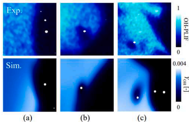
Fig. 17. Time evolution of the flame front during its interaction with ammonia droplets (Reprint from Ref. [126] with permission).
