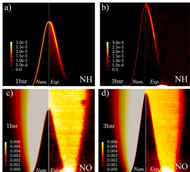
Fig. 5. Spatial distribution of NH and NO at 1 and 3 atm, DNS vs. PLIF (Reprint from Ref. [50] with permission).
