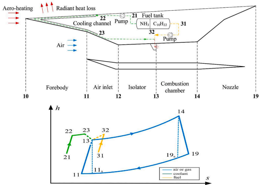
Fig. 18. Thermodynamic model and Enthalpy-Entropy diagram of dual-fuel engine cycle (Reprint from Ref. [131] with permission).
