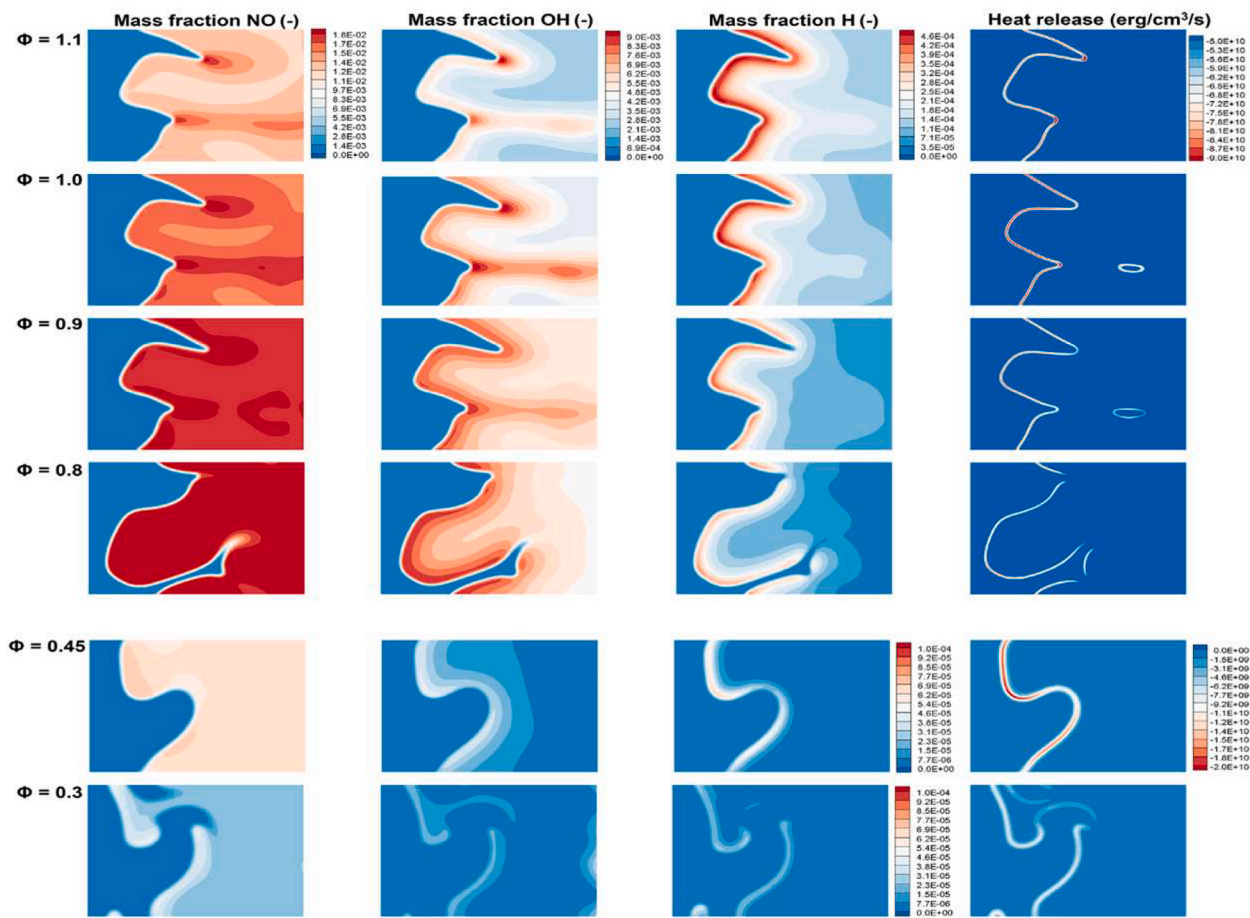
Fig. 4. Wrinkled premixed flame contours showing NO, OH, and H mass fractions (Reprint from Ref. [49] with permission).
