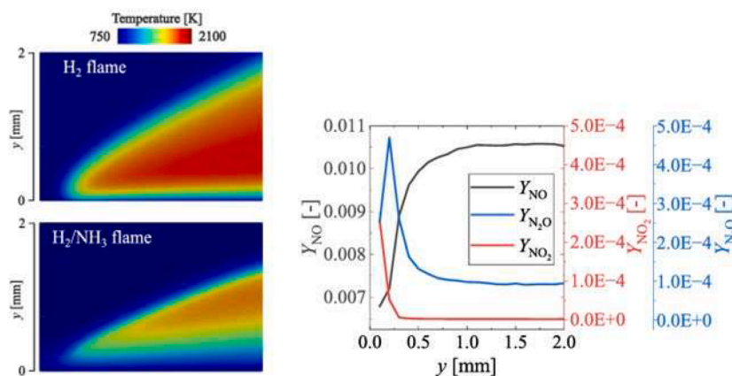
Fig. 10. Left) Instantaneous temperature distribution at z = 15 mm and t = 0.74 ms show the drastic changes in curvature and quenching distance between H_2 and NH_3/H_2 . Right) Emissions and distribution from the wall ( y ) for the NH_3/H_2 blend (Reprint from Ref. [98] with permission).
