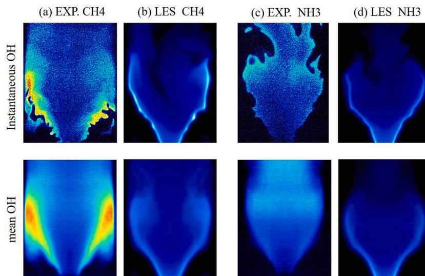
Fig. 8. The comparison of flame structure of \text{NH}_3/\text{air} flame and \text{CH}_4/\text{air} flame. Up: instantaneous OH; down: mean OH (Reprint from Ref. [80] with permission).
