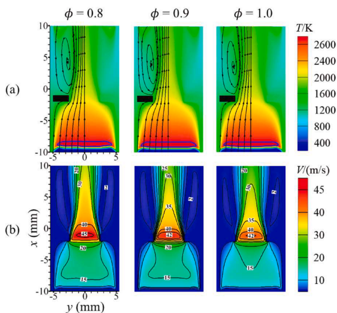
Fig. 3. Contours of temperature, streamlines, and OH mass fraction for varying equivalence ratios (Reproduce from Ref. [48] with permission).
