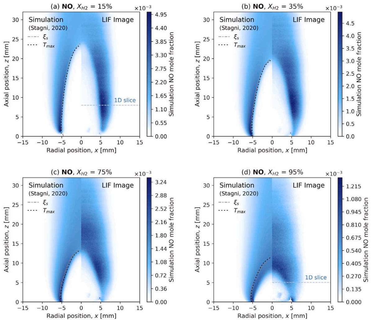
Fig. 7. NO-LIF measurements and simulation comparisons for varying fuel hydrogen ratios (Reprint from Ref. [54] with permission).
