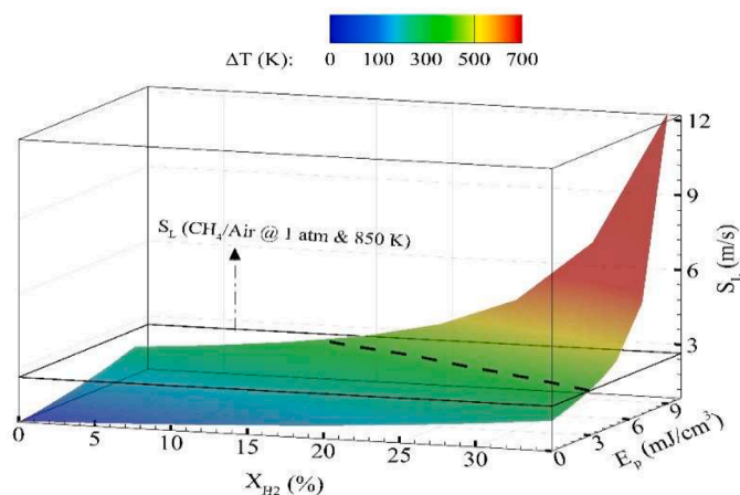
Fig. 22. Laminar flame speed of ammonia as a function of NSD pulse energy density ( E_p ) and mole fraction of hydrogen in the fuel ( X_{\text{H}_2} ), colour-coded with temperature ( \Delta T ). (Reprint from Ref. [161] with permission).
