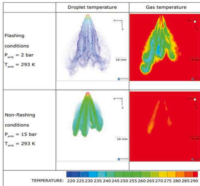
Fig. 12. Simulation showing vapour and droplet formation under flashing and non-flashing conditions (Reprint from Ref. [112] with permission).
