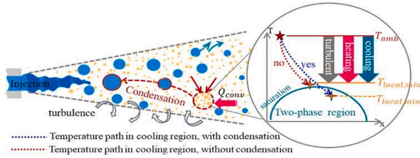
Fig. 14. Competition factors for determining condensation (Reprint from Ref. [121] with permission).
