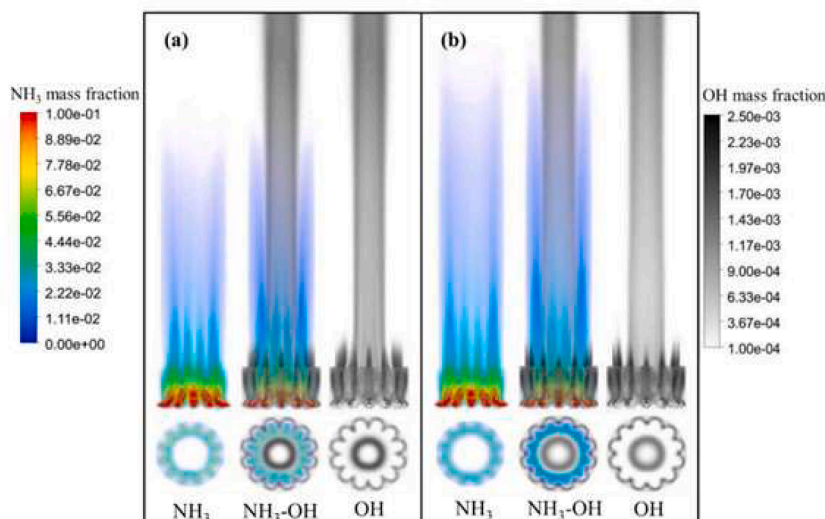
Fig. 19. \text{NH}_3 , \text{NH}_3\text{-OH} , OH distribution in the second stage of the burner (a) without, and (b) with porous media (Reprint from Ref. [139] with permission).
