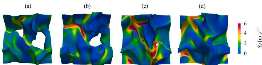
Fig. 24. Turbulent flame front in (a) preheated lean, (b) preheated rich, (c) plasma-assisted lean, and (d) plasma-assisted rich ammonia flames colour-coded with the flame displacement speed (Reprint from Ref. [165] with permission).
