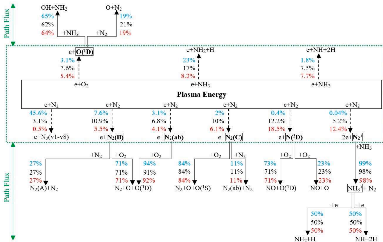
Fig. 21. Main plasma chemical pathways consuming the plasma energy (dashed arrows) and those generating active radicals (arrows) in stoichiometric ammonia/air combustion initially at 850 K, assisted by 20 NSDs with the repetition frequency of 50 kHz and reduced electric field of 100 Td (blue), 350 Td (black), and 700 Td (red). (Reprint from Ref. [162] with permission).
