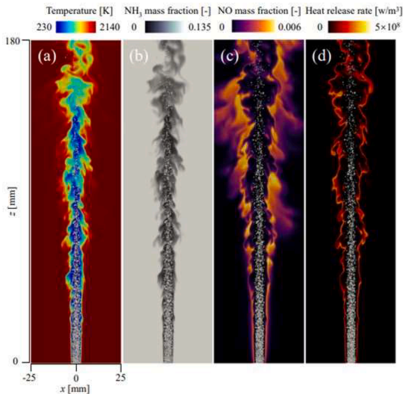
Fig. 16. Instantaneous distribution of a) temperature; b) ammonia mass fraction; c) NO mass fraction, and d) heat release rate. Droplets are shown as white dots (Reprint from Ref. [126] with permission).
