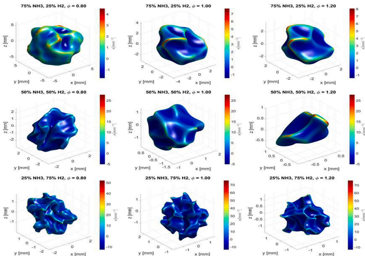
Fig. 2. Flame structures at different equivalence ratios and hydrogen contents (Reprint from Ref. [16] with permission).
