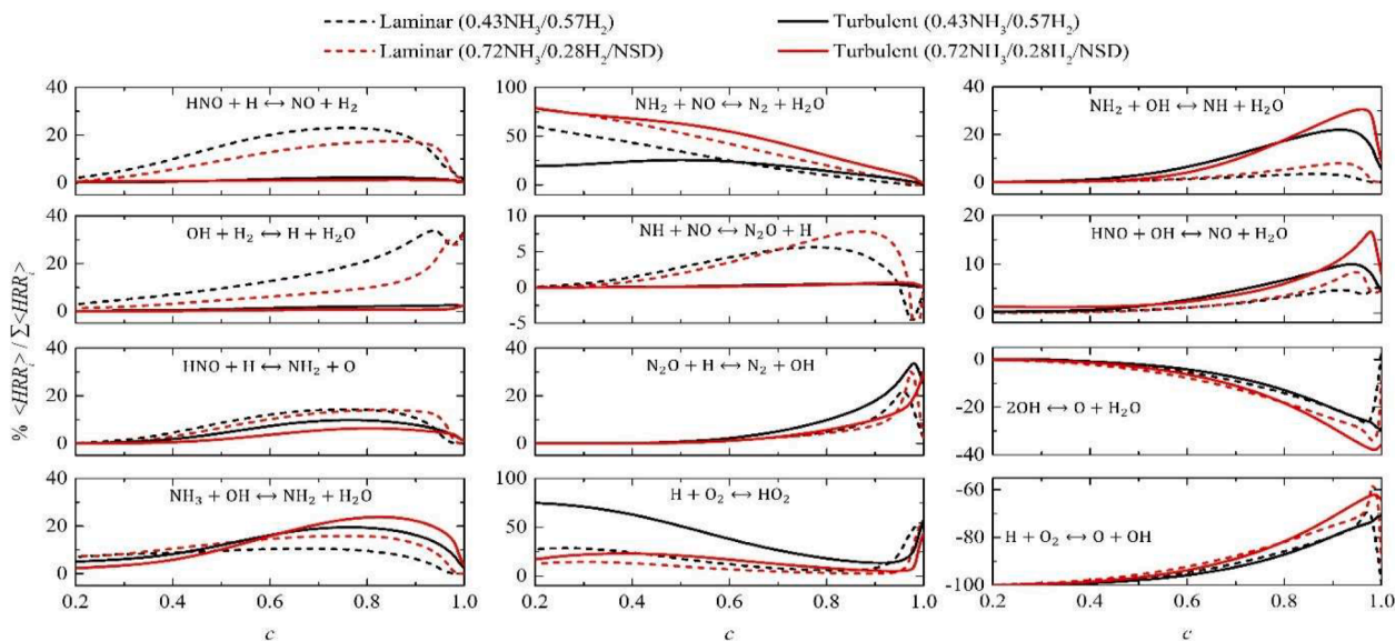
Fig. 23. Key chemical reactions contributing to heat release in laminar and turbulent ammonia/hydrogen/air flames (Reprint from Ref. [153] with permission).
