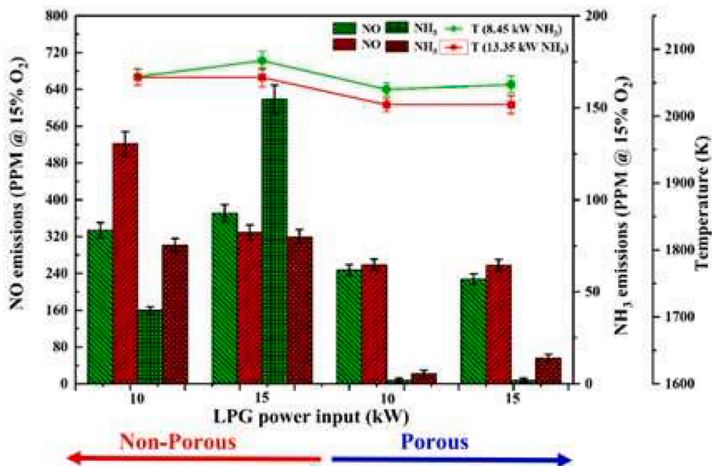
Fig. 20. Comparison of measured NO, NH 3 and exit temperature of the burner with and without porous foams at various thermal inputs under stoichiometric conditions (Reprint from Ref. [139] with permission).
