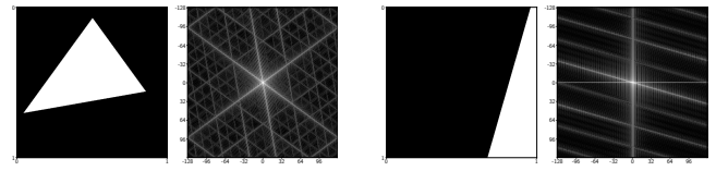
Figure 2: Two integrands with discontinuities and their respective power spectra. The power spectra show high-energy directions perpendicular to the orientation of the discontinuity. Due to the finite integration domain and as the Fourier transformation operates on a toroidally, the second integrand also has discontinuities along the horizontal and vertical axes that are visible in the power spectrum.
