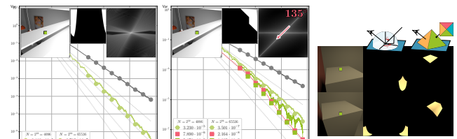
Figure 12: Hemispherical sampling: an octahedral (right plot) instead of an angular mapping (left plot) keeps edges in the integrand straight, and thus the energy in the power spectrum focused in one direction. This means our aligned sampling points significantly improve the variance. Right: examples of integrands using angular mapping (center) or octahedral mapping (right). The energy is no longer spread across a range but into multiple discrete directions.
