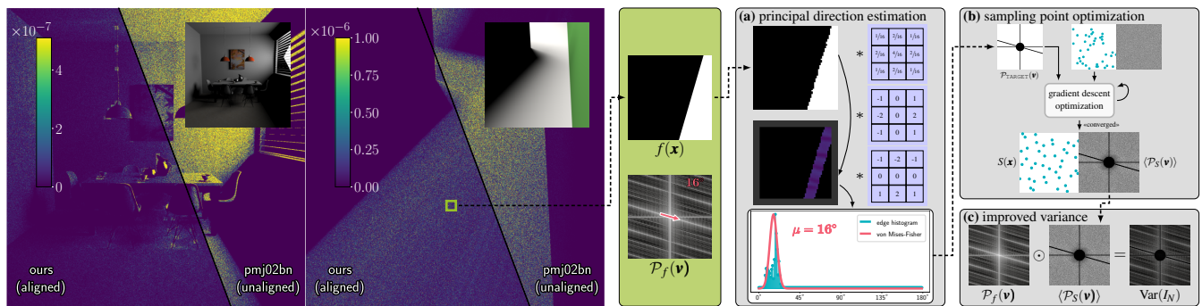
Figure 1: We improve the variance convergence rate of the Monte Carlo estimator in offline path tracing on two-dimensional discontinuous integrands. To that end, we (a) sparsely sample the integrand f(\mathbf{x}) in blocks of pixels to construct a histogram of occurring edge directions. We estimate principal directions in the power spectrum \mathcal{P}_f(\mathbf{v}) (red arrow) from the histogram, as principal directions in \mathcal{P}_f(\mathbf{v}) are perpendicular to edges in f(\mathbf{x}) . (b) We optimize a set of sampling points S(\mathbf{x}) with an anisotropic spectrum that matches the estimated spectrum of the integrand. (c) Using our aligned points improves the convergence rate compared to existing unaligned anisotropic sampling patterns.
