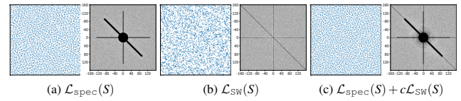
Figure 3: Three synthesized point sets and their respective power spectra, optimized for different loss functions using our gradient-based optimization. (a) The power spectrum loss \mathcal{L}_{\text{spec}}(S) suppresses a finite set of frequencies. (b) The sliced Wasserstein loss \mathcal{L}_{\text{SW}}(S) ensures stratification for a given set of directions. (c) We combine both losses to synthesize points with both properties.
