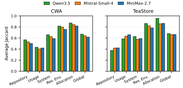
Figure 3: Average Jaccard per PCM view (mean over use cases and runs) for the three evaluated LLMs on CWA and TeaStore.
