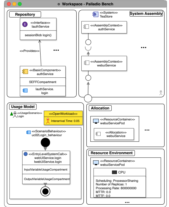
Figure 2: Generated PCM instance for a login scenario
