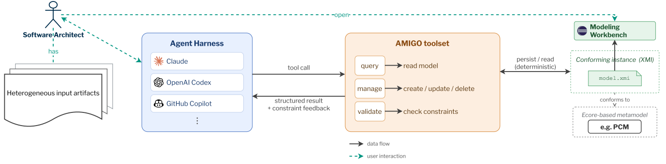
Figure 1: AMIGO architecture. A software architect interacts with an agent harness. The agent expresses modeling intent through tools over the Model Context Protocol (MCP), which executes operations deterministically and persists a conforming model instance. The persisted instance conforms to a pluggable Ecore-based metamodel and opens in the modeling workbench.
