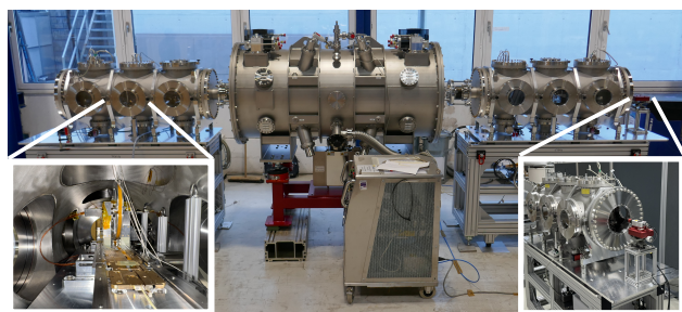
Figure 3: Mobile Measurement system with the latest wiggler for Diamond Light Source, UK. Bottom left: sledge and instrumentation. Bottom right: laser interferometer.
