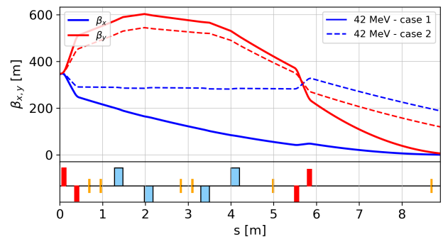
Figure 2: Beta functions after the linac (0 m in the plot corresponds to 7.05 m in FLUTE) at 42 MeV for two example sets of quadrupole parameters. Case 1: focused resulting in \beta_x=1.6 m, \alpha_x=1.8 , \beta_y=0.3 m, \alpha_y=0.9 . Case 2: example for bigger final sizes with \beta_x=188 m, \alpha_x=20 , \beta_y=119 m, \alpha_y=19 .
