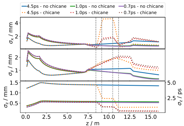
Figure 6: Different operation parameters for 300 pC. The laser pulse length is varied from 0.7 ps to 4.5 ps reducing the transverse size increase in the low energy section. Options with and without the chicane (set to a moderate shortening) are shown.
