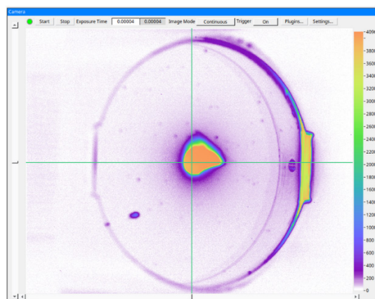
Figure 6: Beam profile with a charge of 450 pC and energy of 56 MeV on the screen after the bunch compressor.
