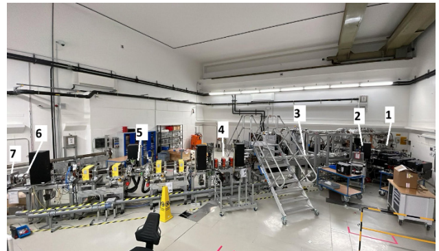
Figure 5: Overview of the FLUTE accelerator: 1 – RF photoinjector, 2 – first diagnostic section, 3 – linac, 4 – quadrupole triplet, 5 – magnetic chicane (bunch compressor consisting of four dipole magnets), 6 – in-air experiment section, 7 – beam dump.
