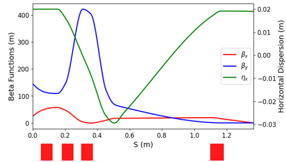
Figure 7: Optical functions along Matching Cell II.
