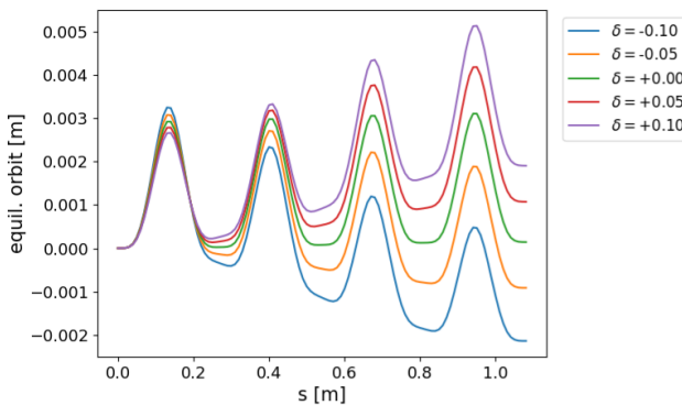
Figure 5: Particle trajectories in the FFA-based dispersion creator for different relative momenta \delta .
